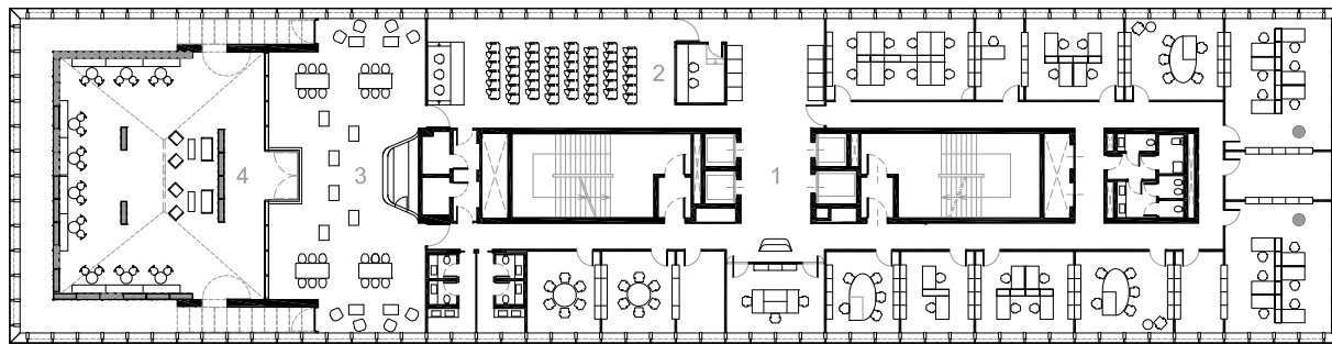
Plan Floor +18.56m 1. Offices 2. Press Room 3. Event Area 4. Terrace
