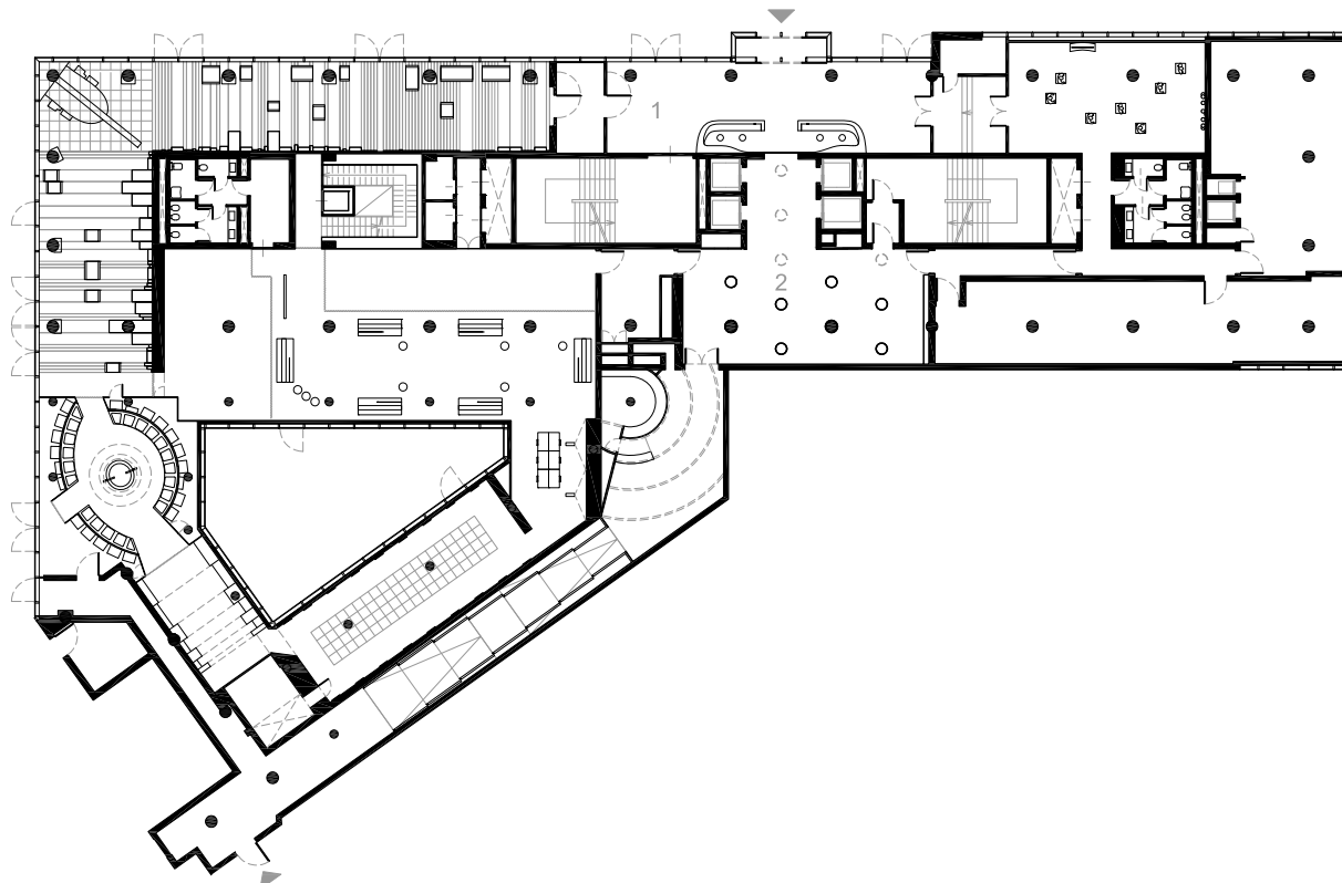
Plan Floor -00.48m 1. Mondo Milan - museum 2. Lower level Hall
