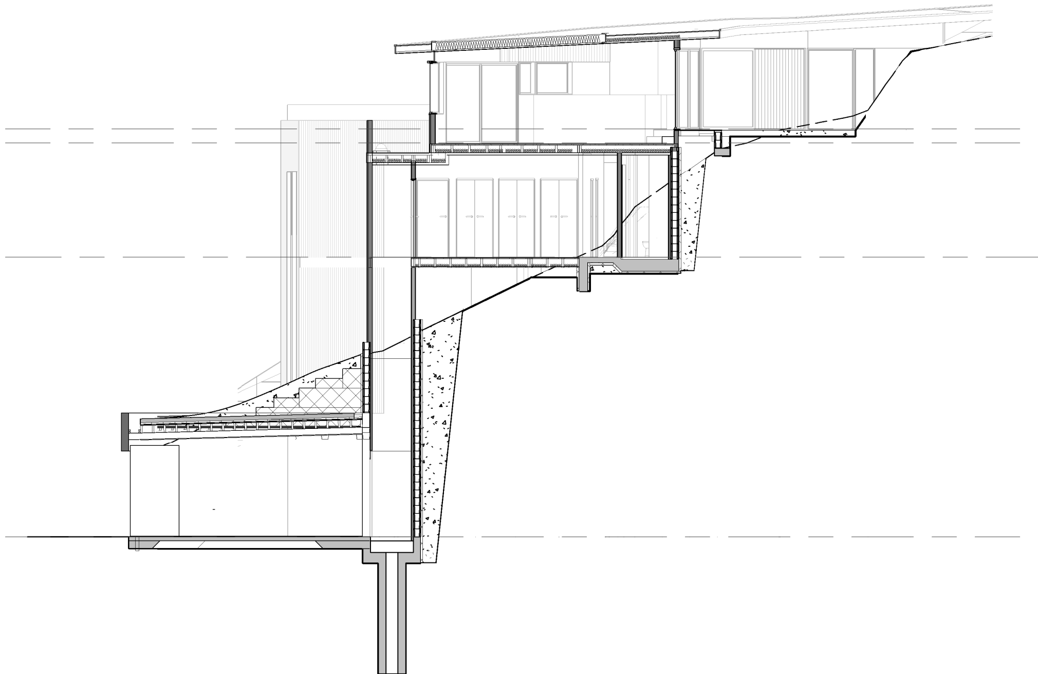
TYPICAL SECTION scale 1:100
