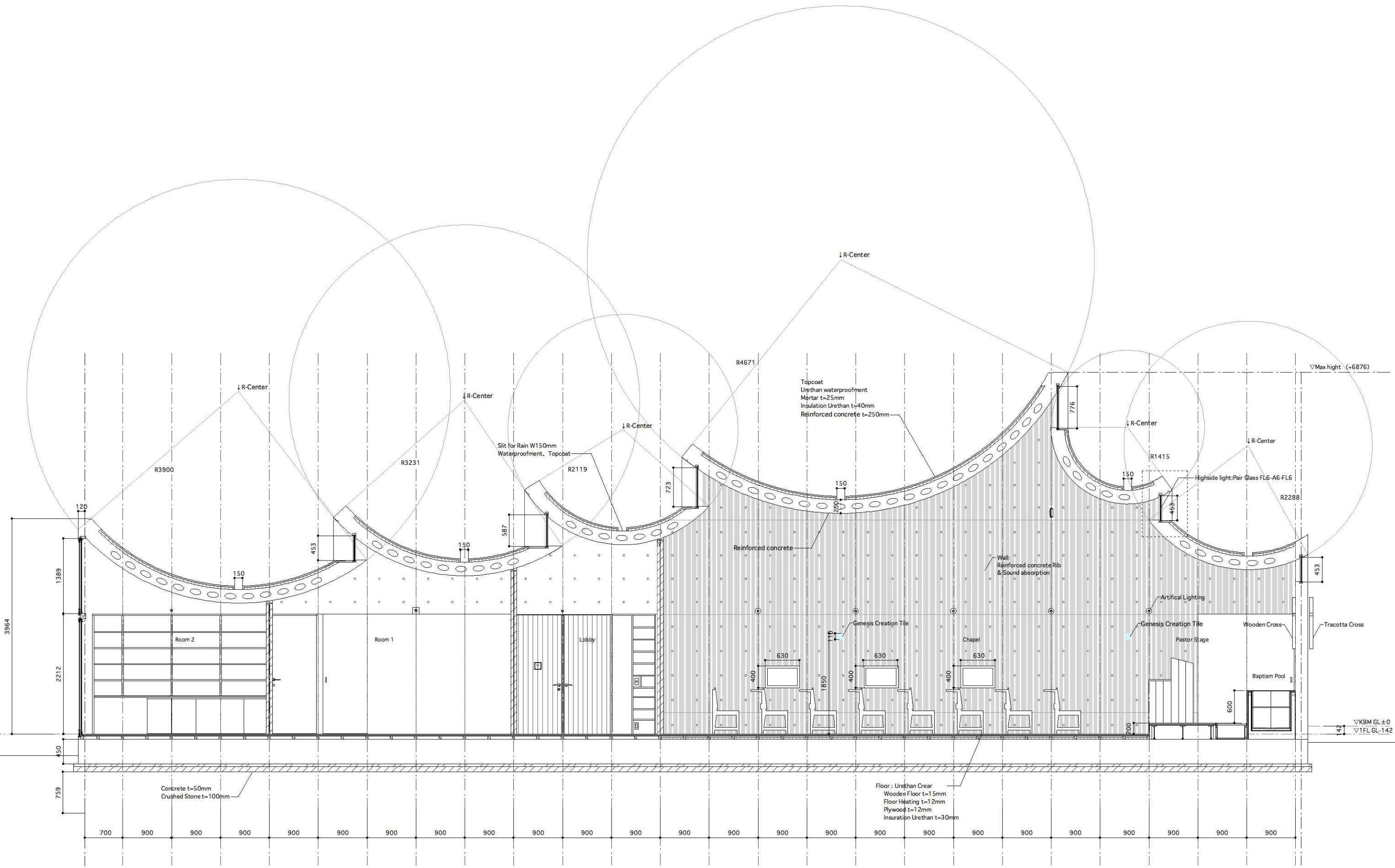
Section S=1:65
