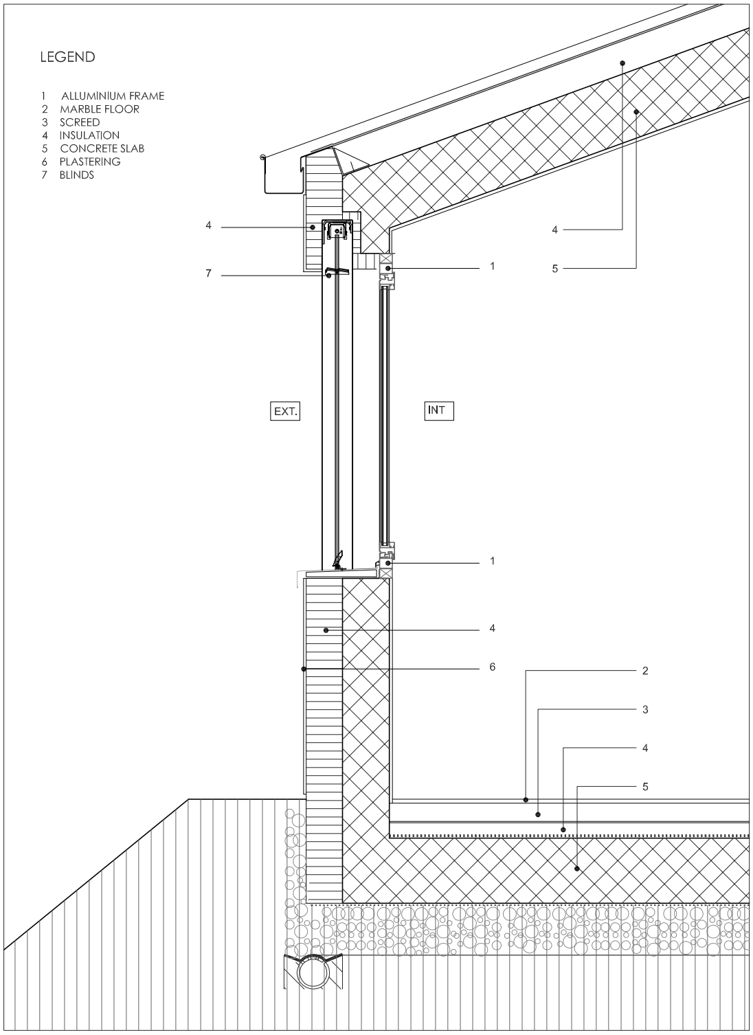
DETAIL 3 - SECTION VIEW
