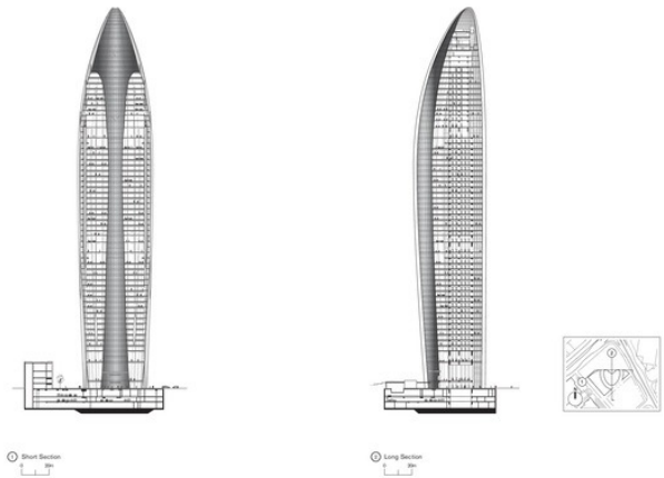
Project Name National Bank of Kuwait Filename 2184_FP725430.pdf Caption Presentation section drawing Copyright holder Foster + Partners
