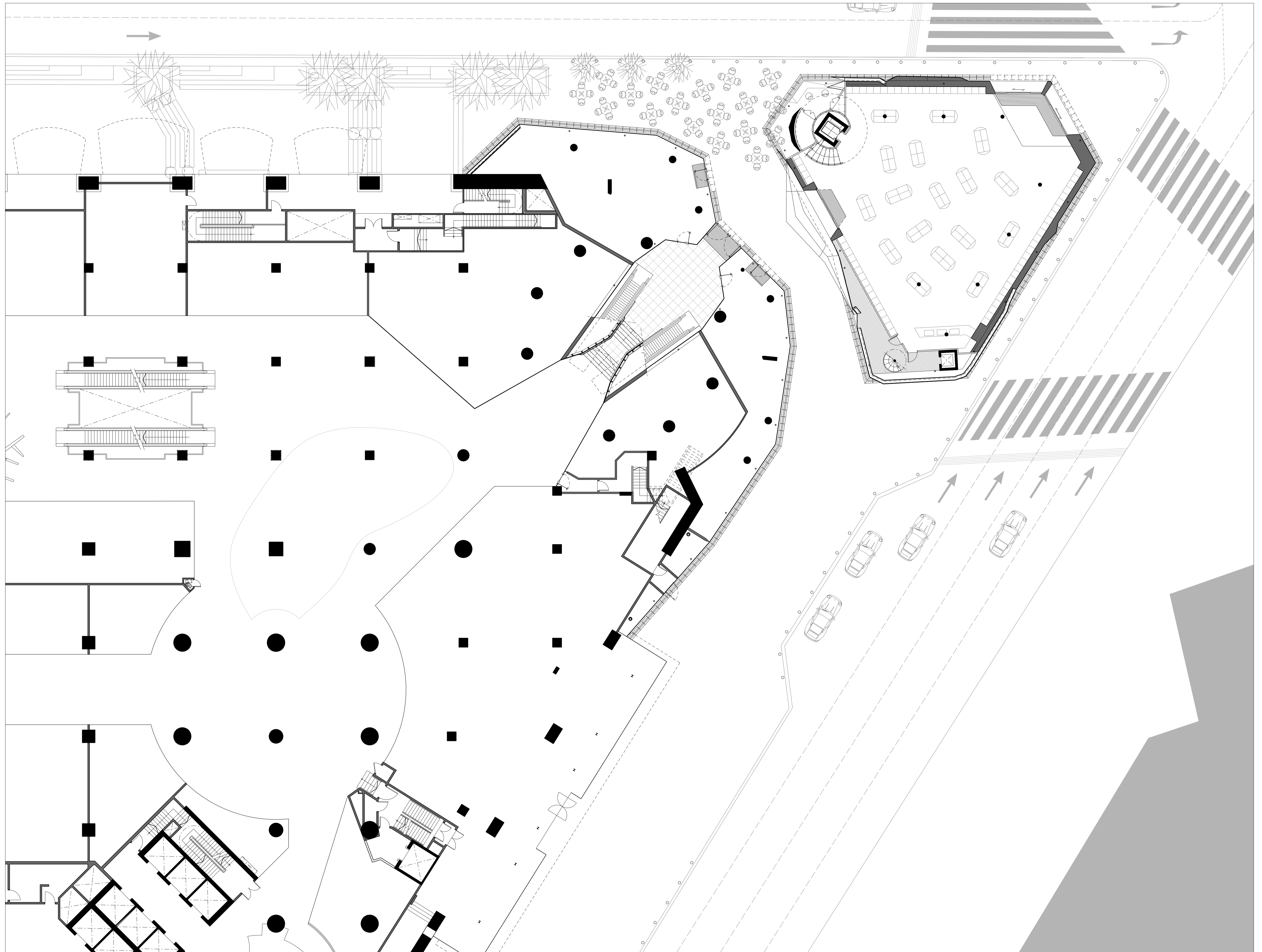
GENERAL ARRANGEMENT / PLAN LEVEL MAIN ENTRANCE
