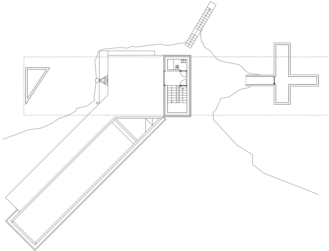
Floor plan -1
