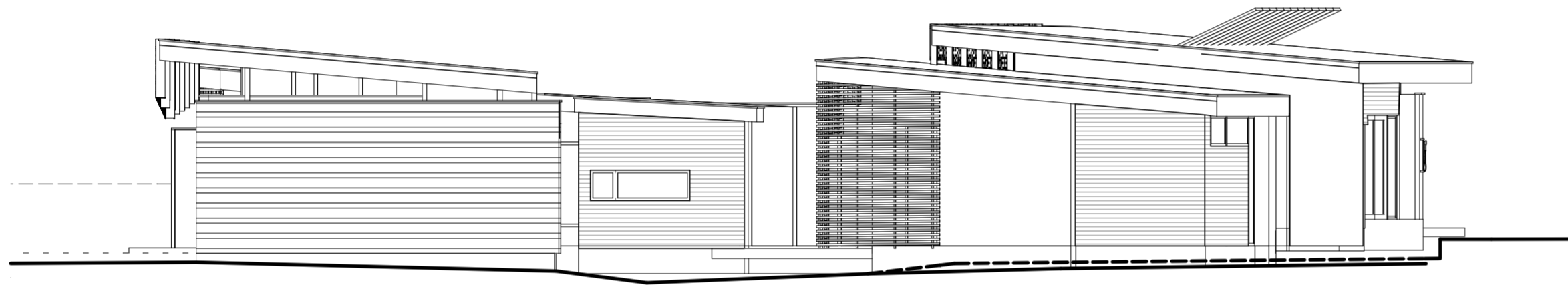
West Elevation
