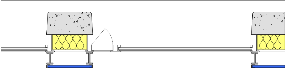
Façade type 4: - South façade, operable windows, partial shading, PV panels generating sustainable energy
