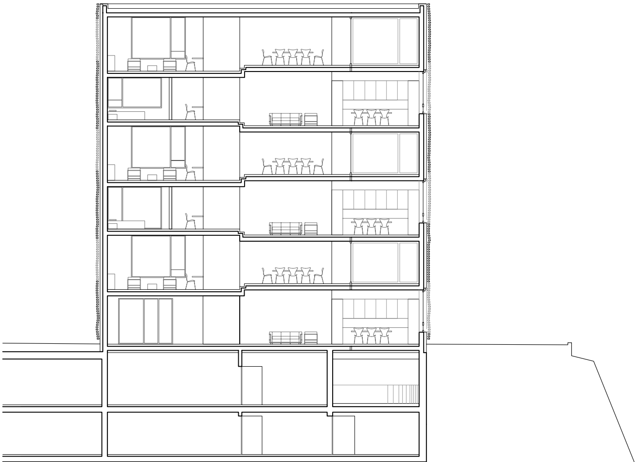
Longitudinal section _ building B 1:200
