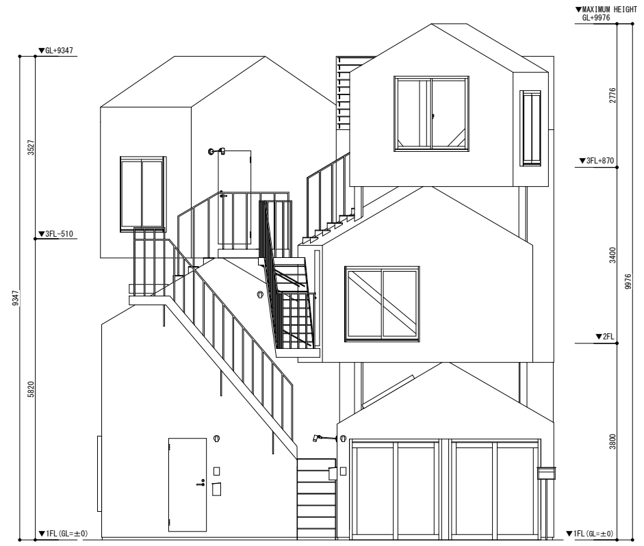
NORTH ELEVATION
