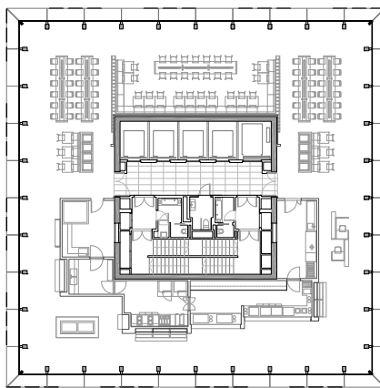
PLANTA SEGUNDA / SECOND FLOOR PLAN
