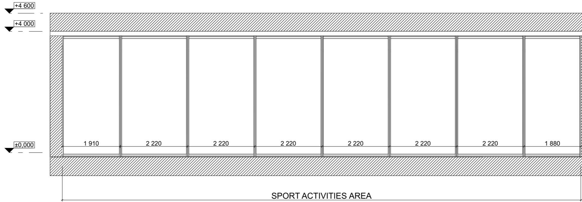
S21 SECTION
