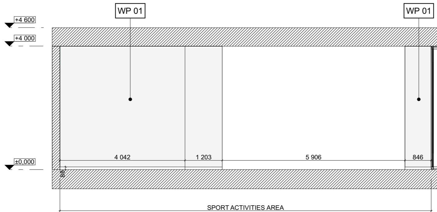
S22 SECTION
