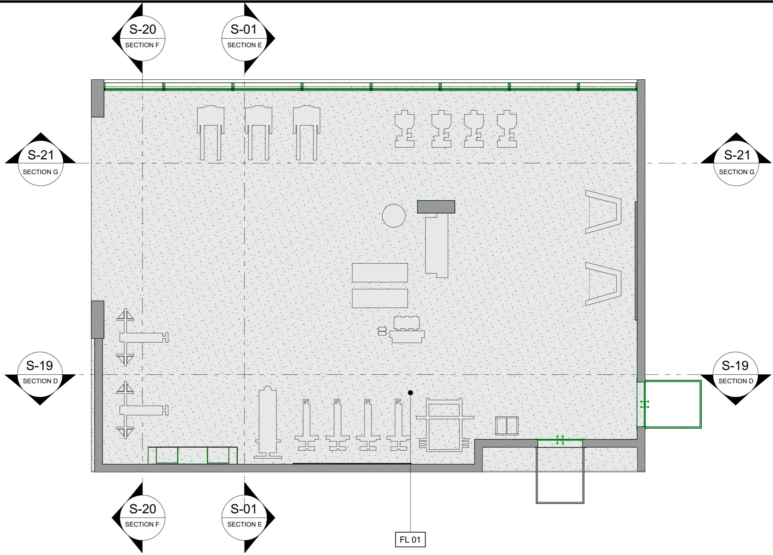
4 B06 - SPORT ACTIVITIES - FLOORING PLANE FLOORING SCALE 1:75 M
