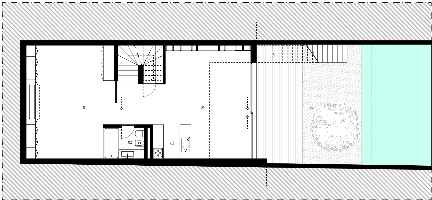
BASEMENT PLAN
