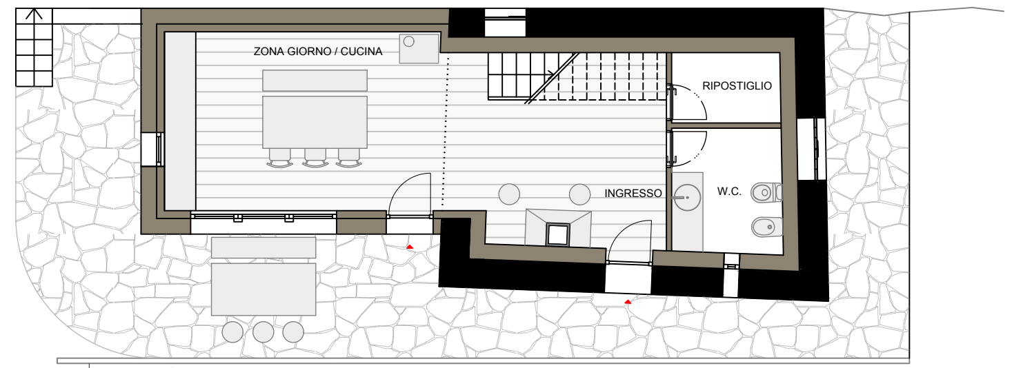
PIANO TERRA
