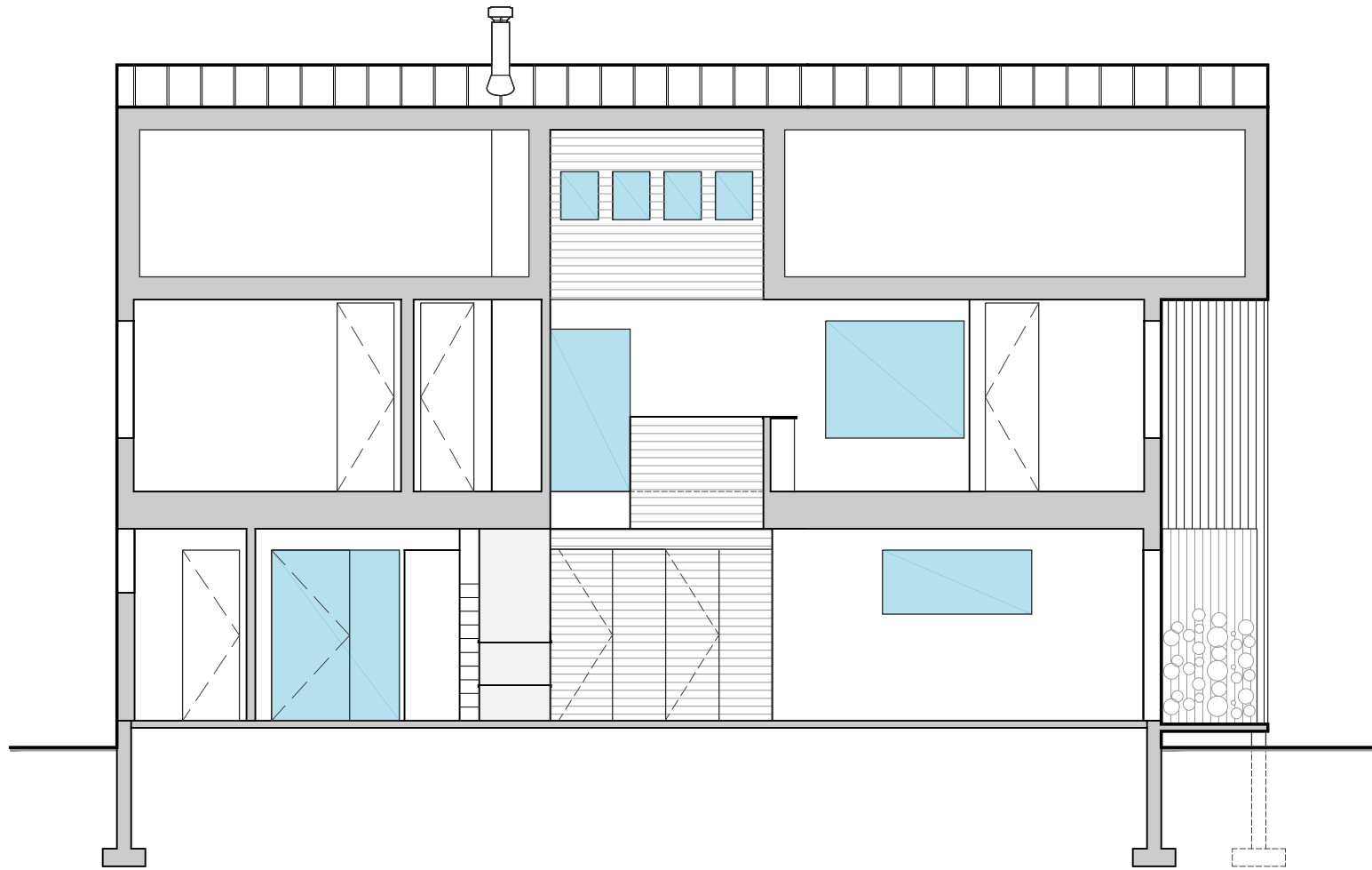
SECTION XX
