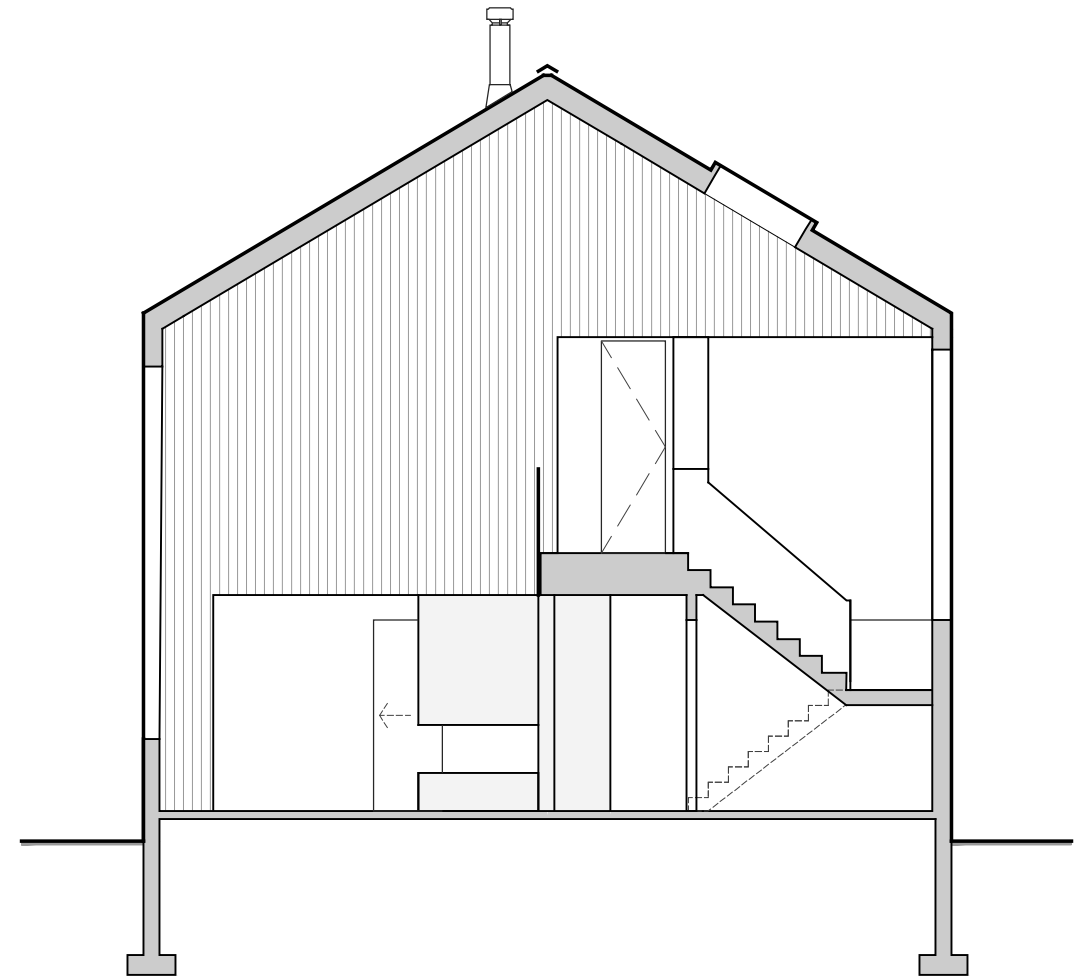
SECTION YY
