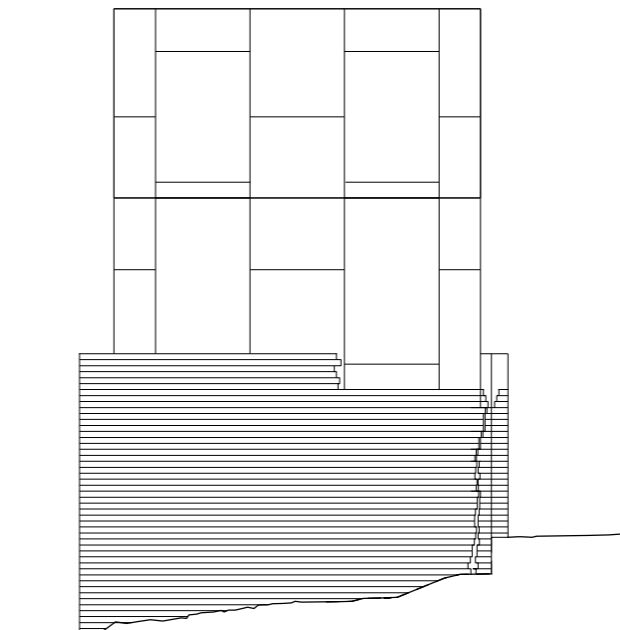
SOUTH ELEVATION
