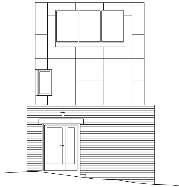
NORTH ELEVATION
