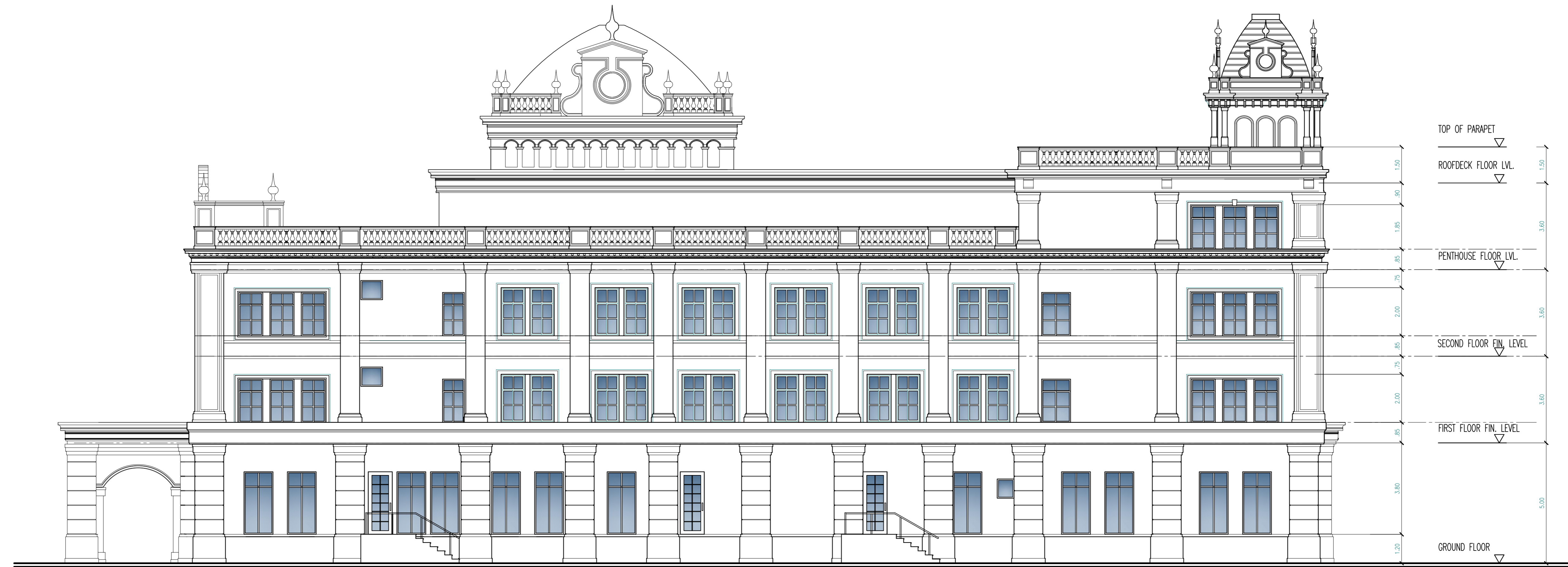
1 A/3 SCALE 1:100 M. LEFT SIDE ELEVATION BUILDING -B
