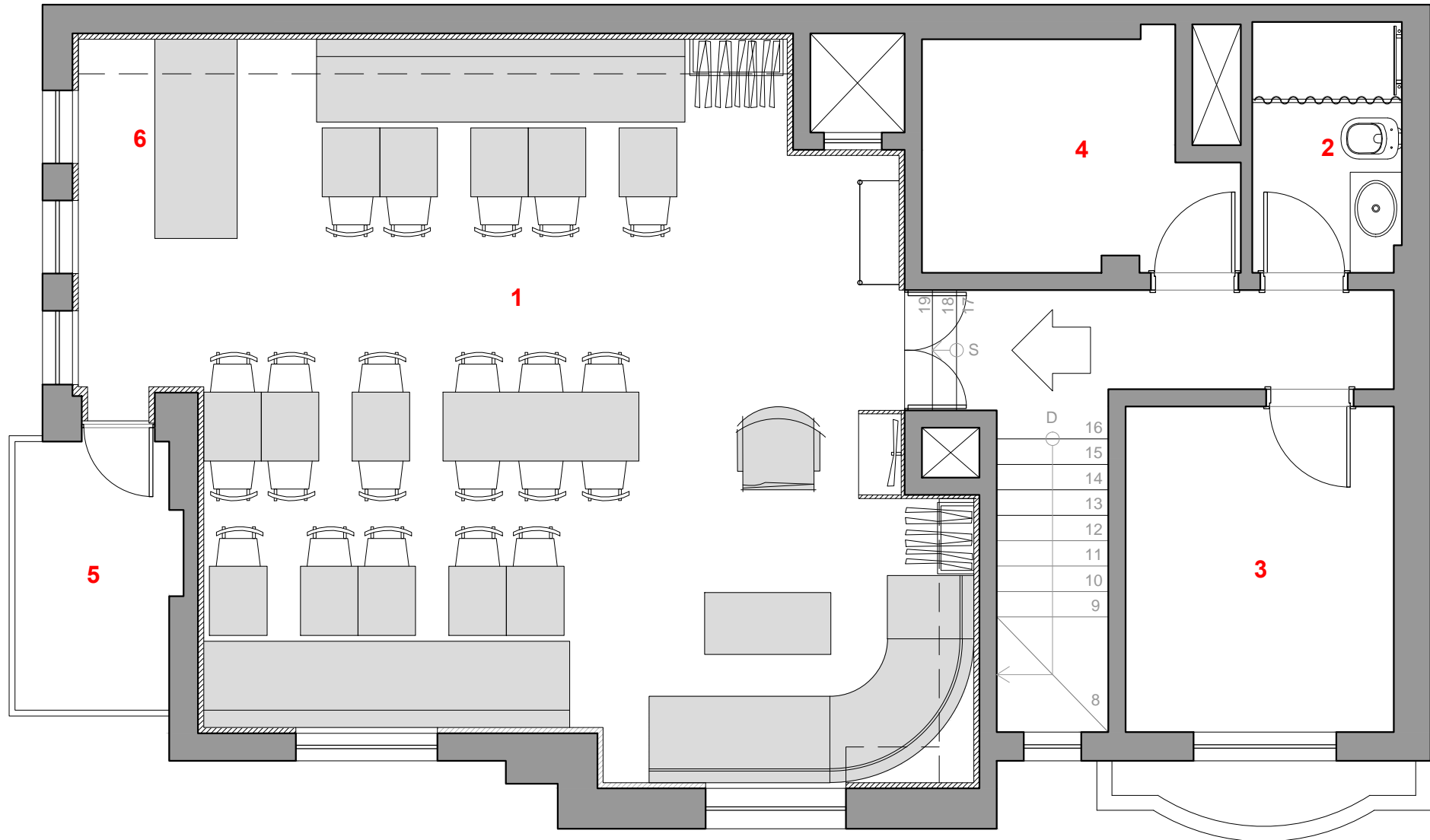
1 Floor Plan
