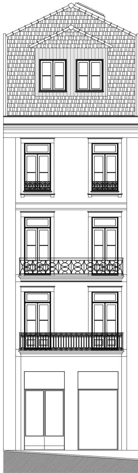
Street facade
