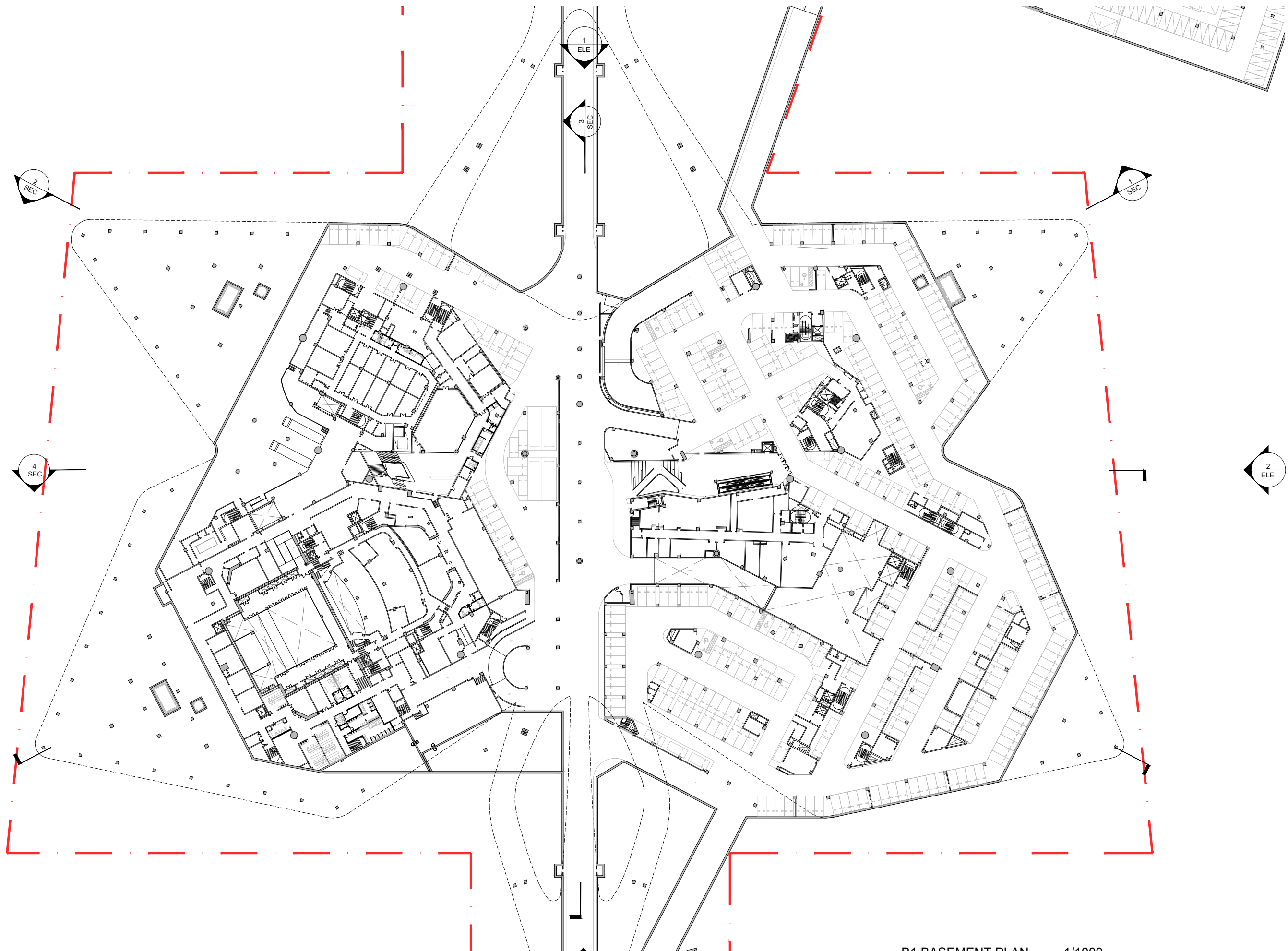
B1 BASEMENT PLAN 1/1000
