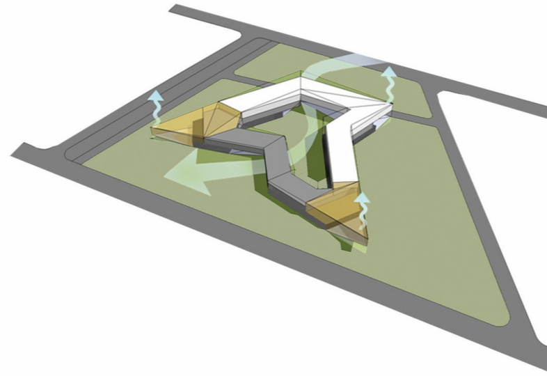
Built volume lifted from the ground at the southwest and northeast sides to facilitate south westerly breeze through the courtyard.
