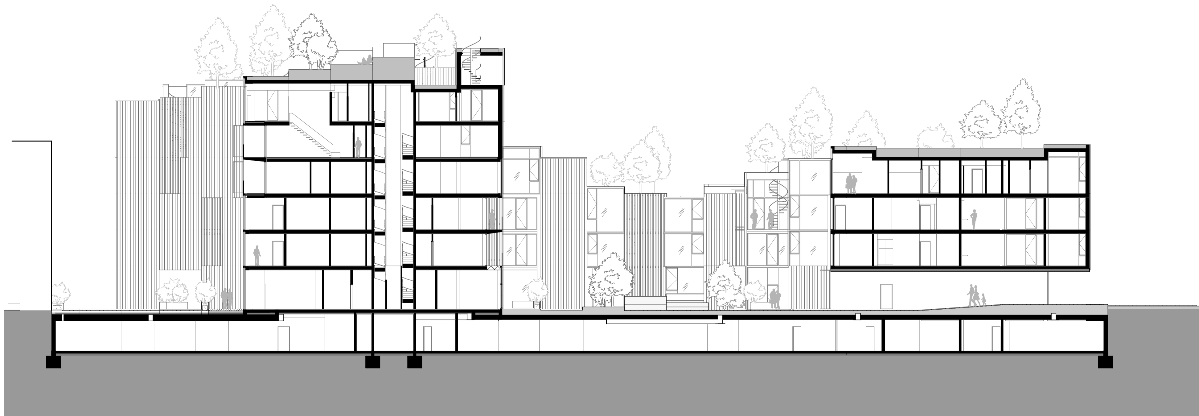
SECTION B-B
