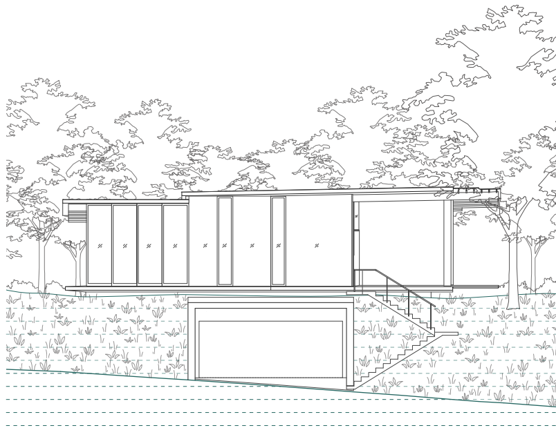
south elevation s=1/200
