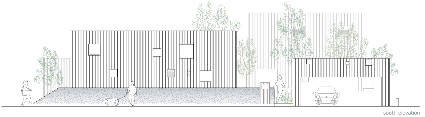
south elevation
