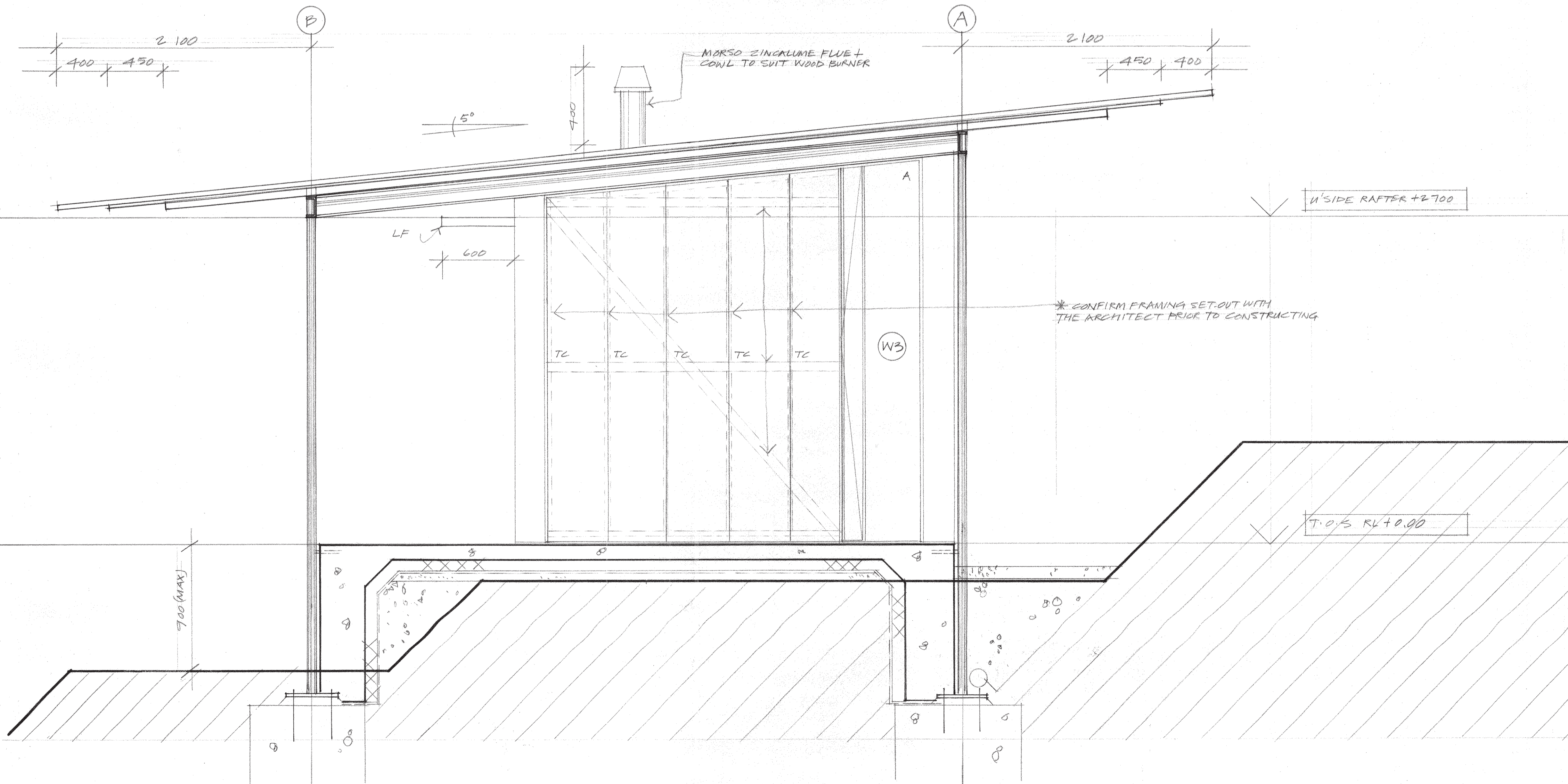
SECTION 1:20
