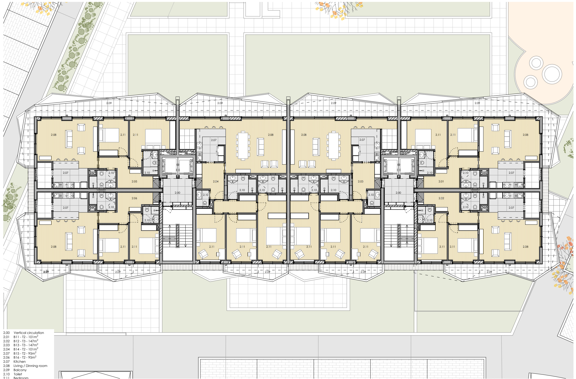
BUILDING B - TYPICAL FLOOR PLAN (2ND FLOOR)
