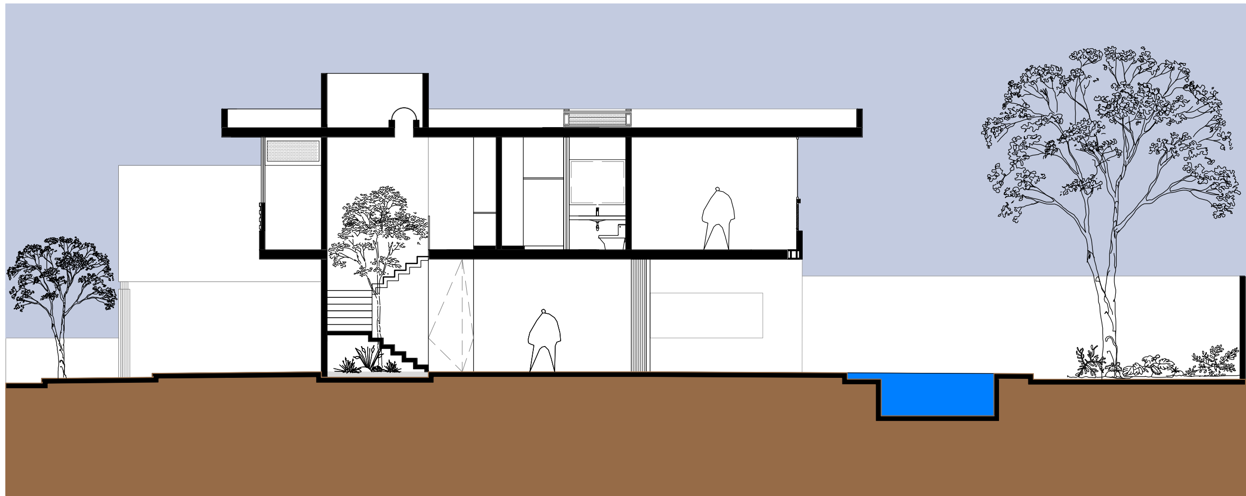
SECTION B-B'
