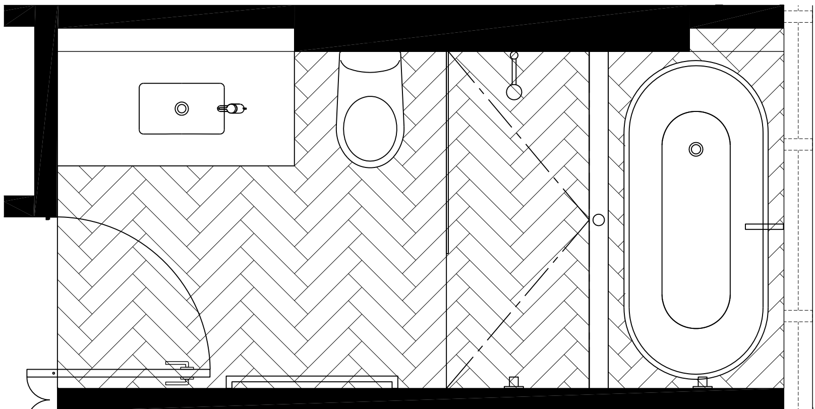
BATHROOM PLAN
