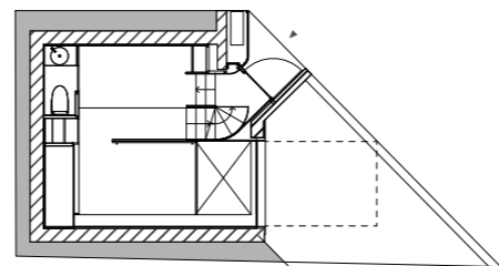
B1F PLAN
