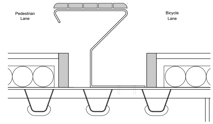
Chengdu Jiangxi River Bridge Bench Details 0 50cm 100cm
