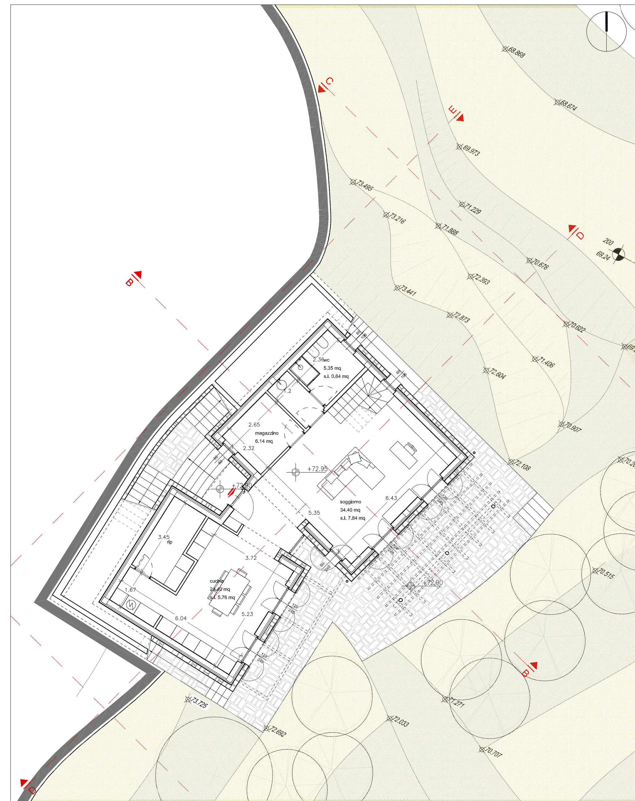
piano terra 1_100
