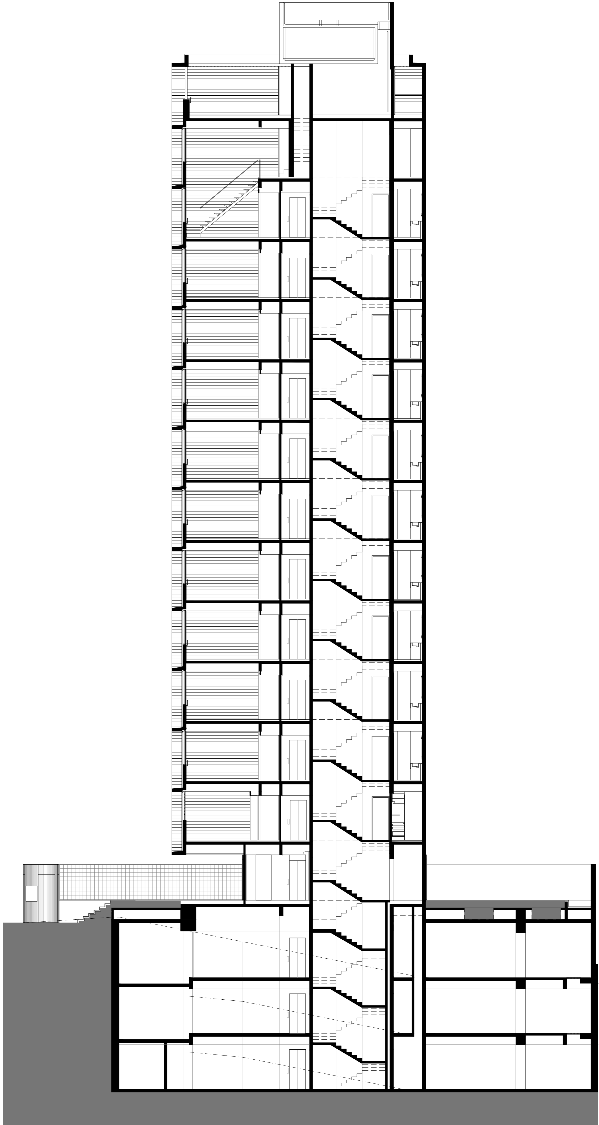
corte aa _ aa section 1:100 0 1 5m
