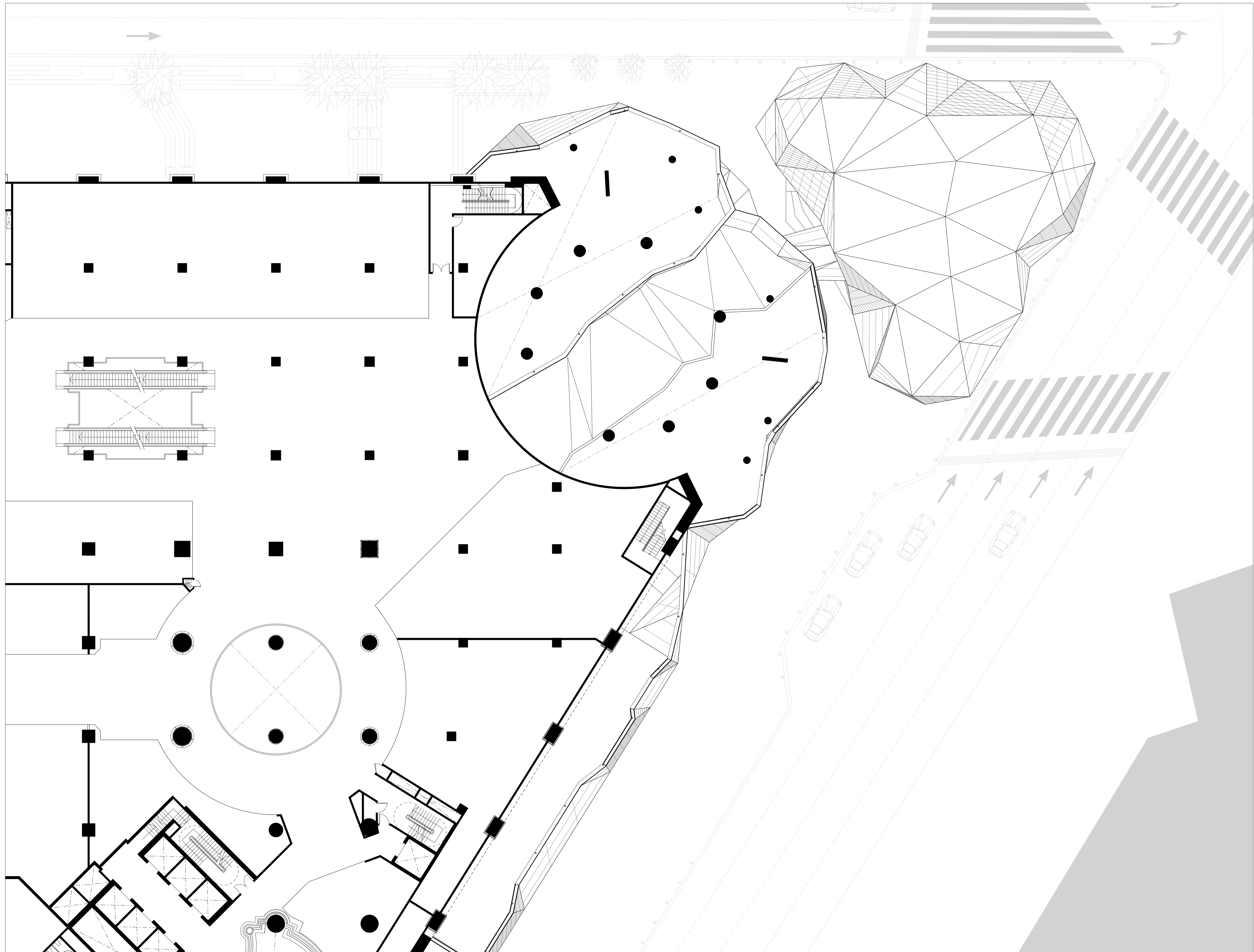
1 GENERAL ARRANGEMENT / PLAN LEVEL 6 GA/p104 SCALE 1:150
