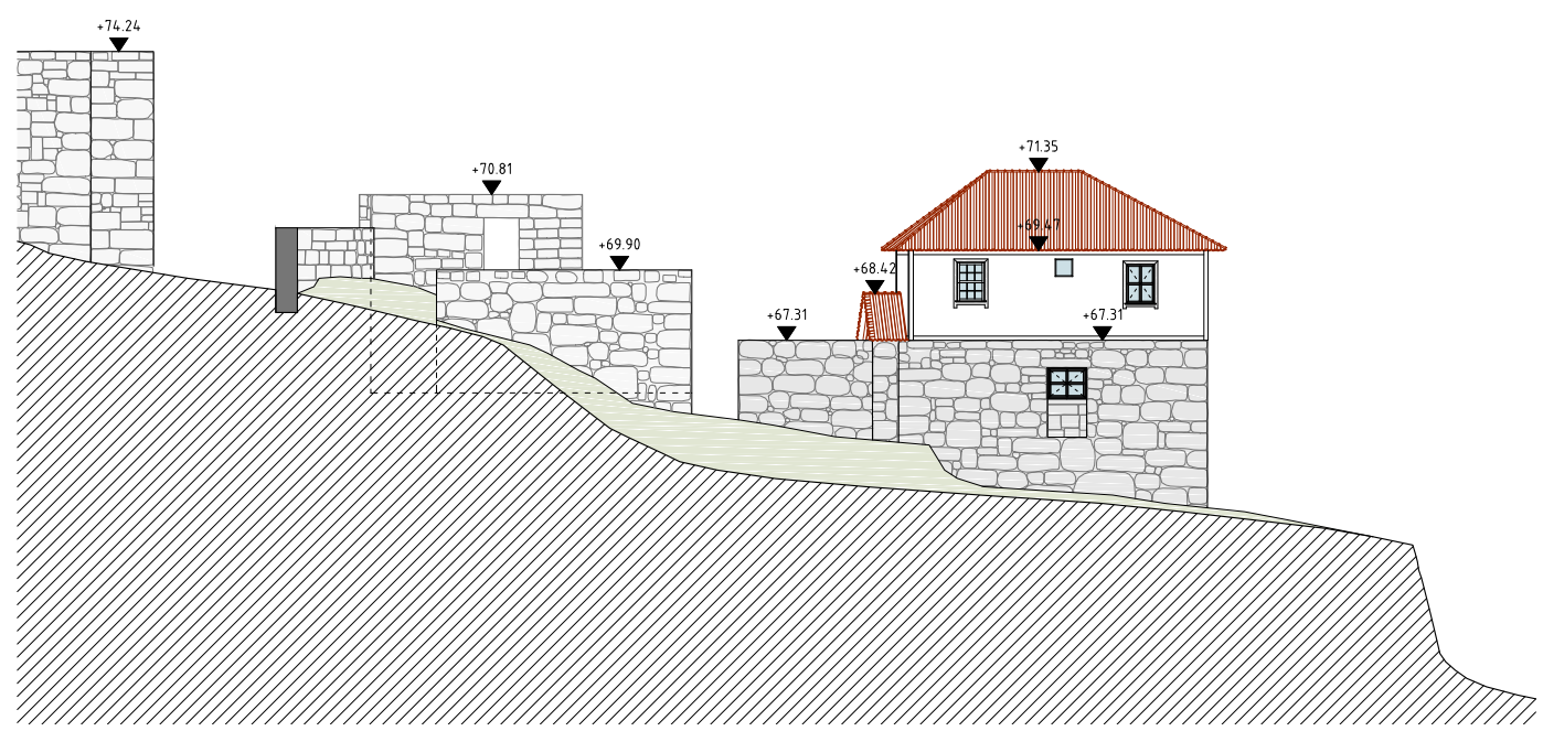
SECTIONS A AND B
