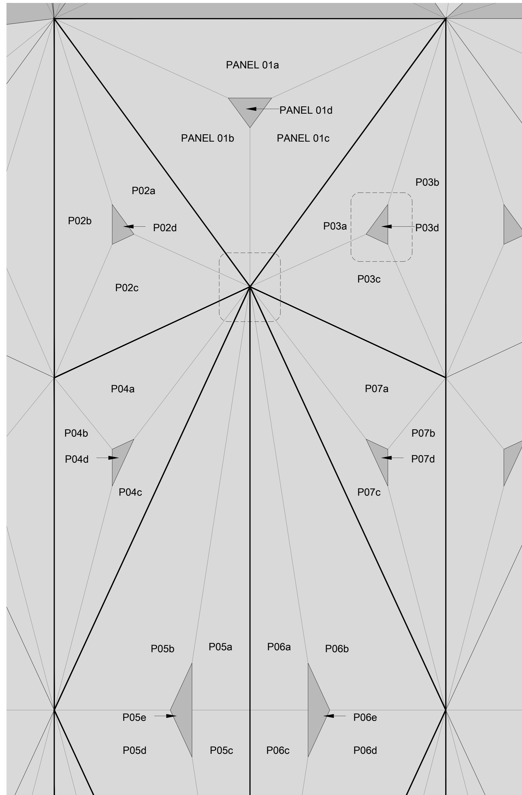
L19 & 28 TRIANGULATED CEILING PANEL LAYOUT
