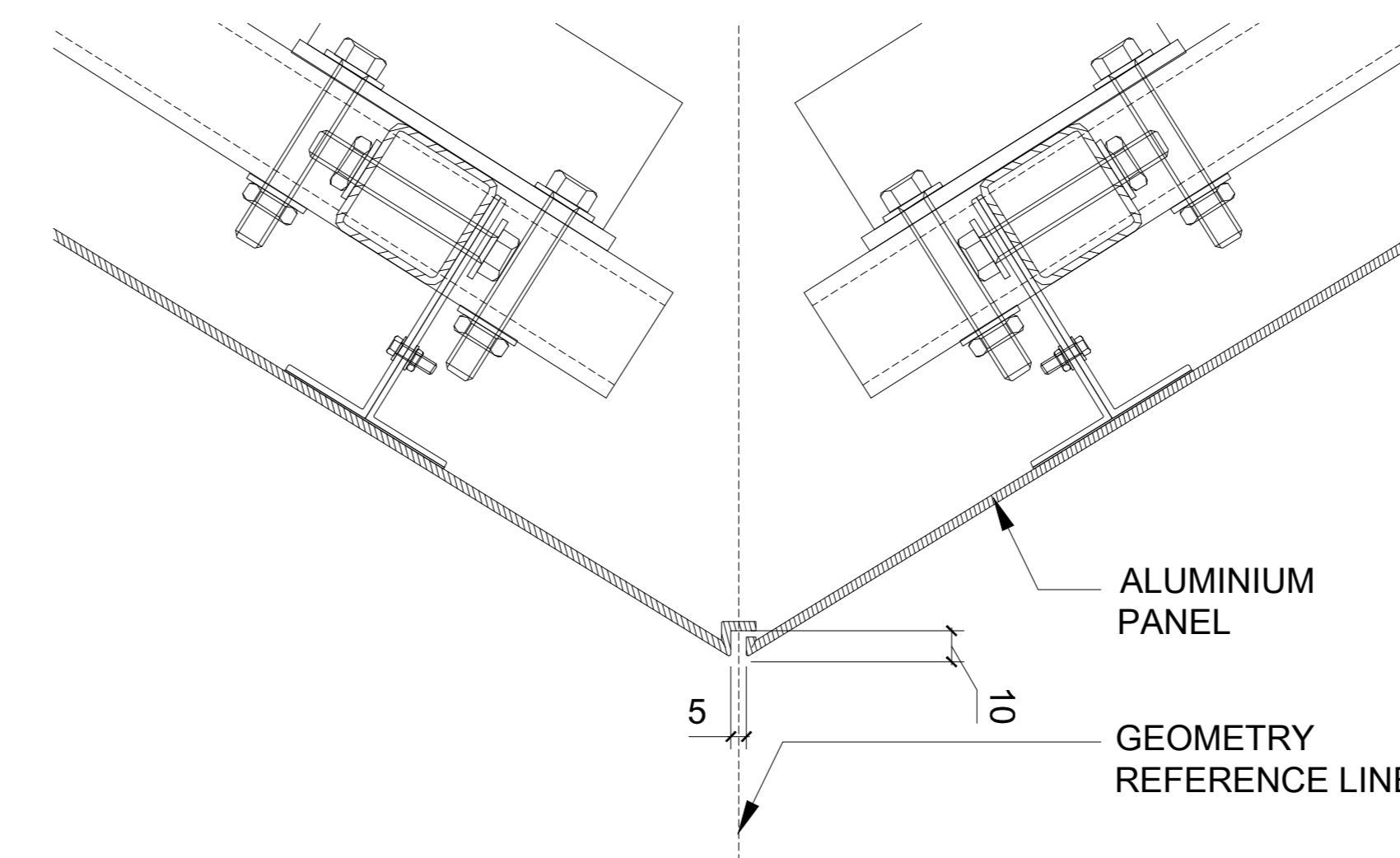
PANEL RECESSED JOINT TYPE 03
