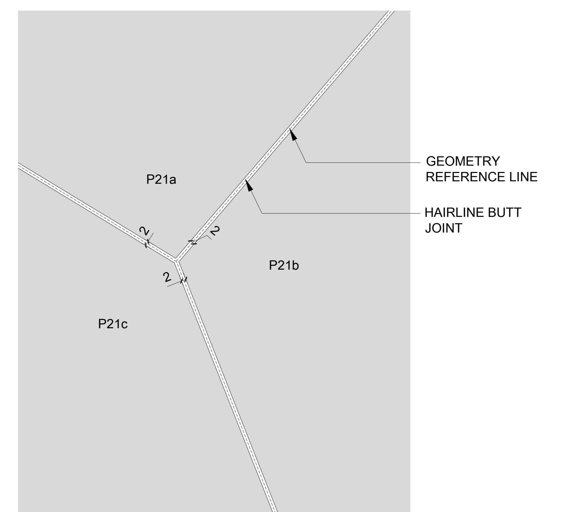
TRIANGULATED PANELS JUNCTION
