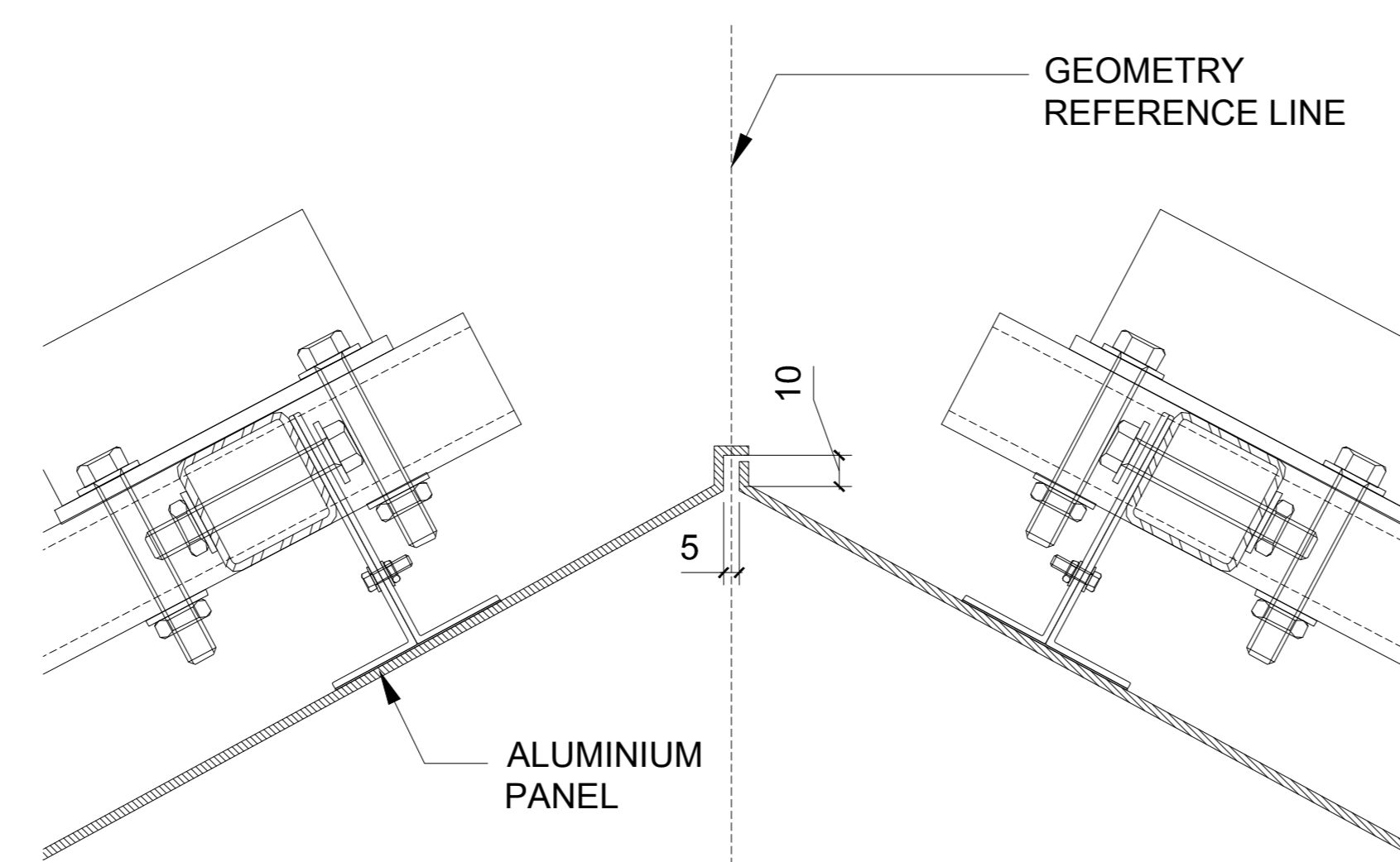
PANEL RECESSED JOINT TYPE 02
