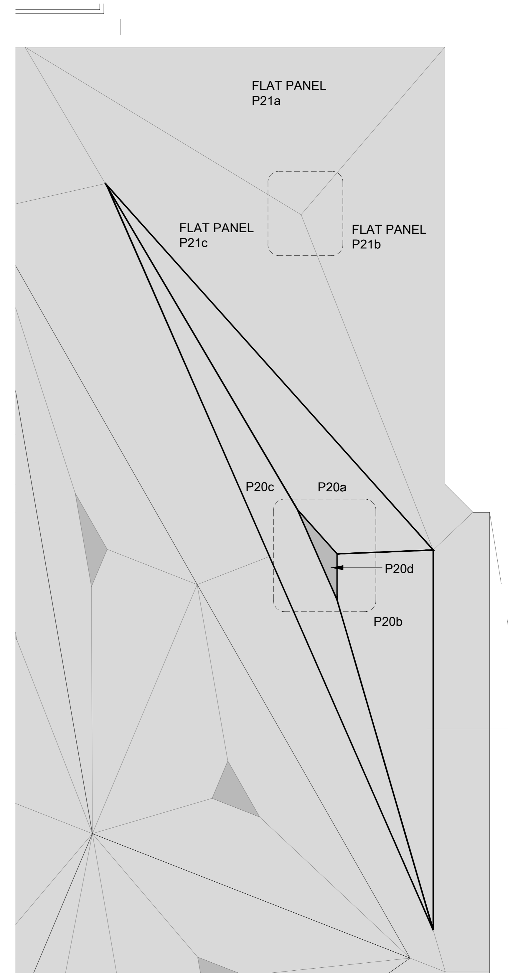
L38 TRIANGULATED CEILING PANEL LAYOUT
