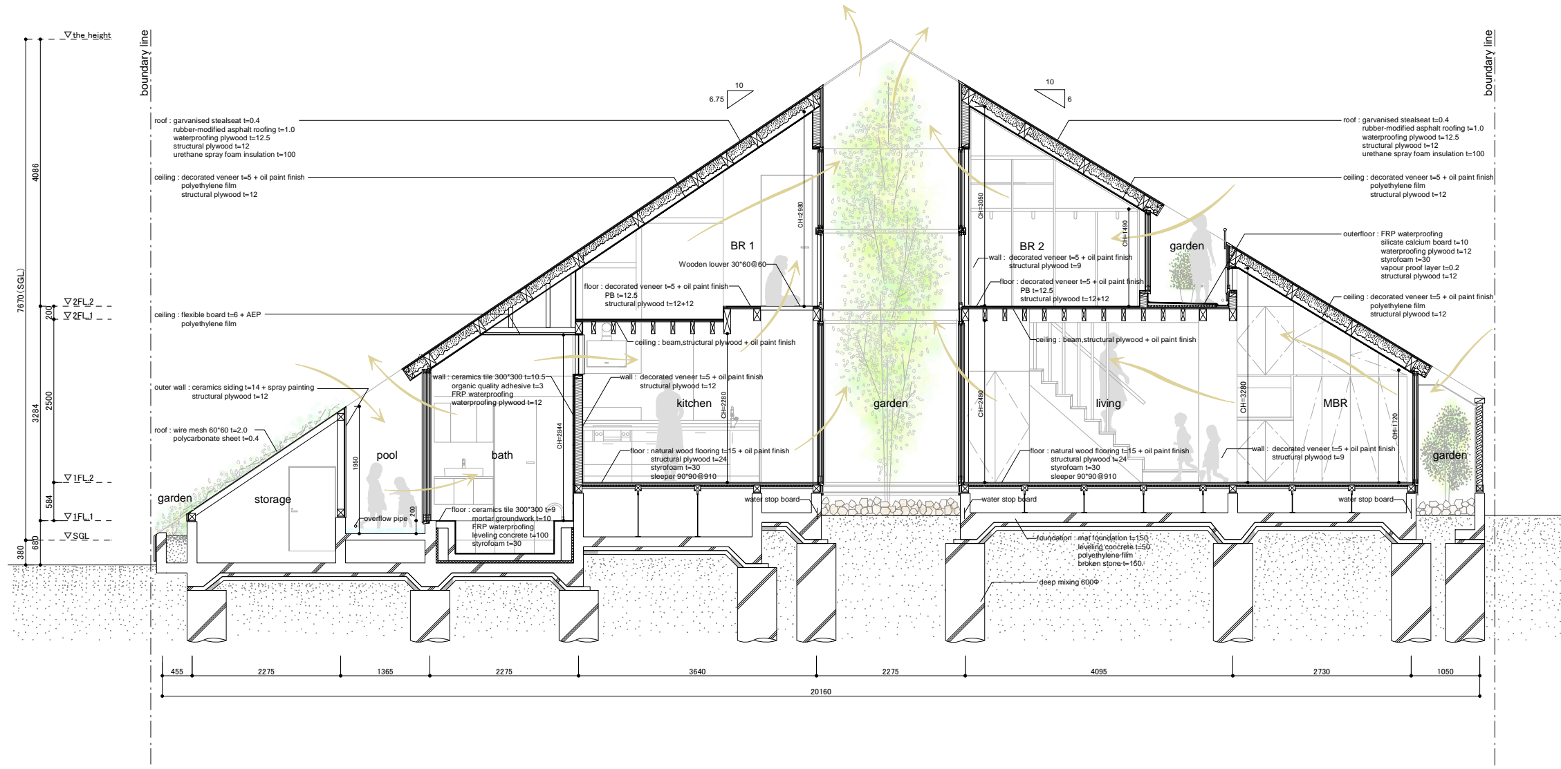
SECTION 1:80
