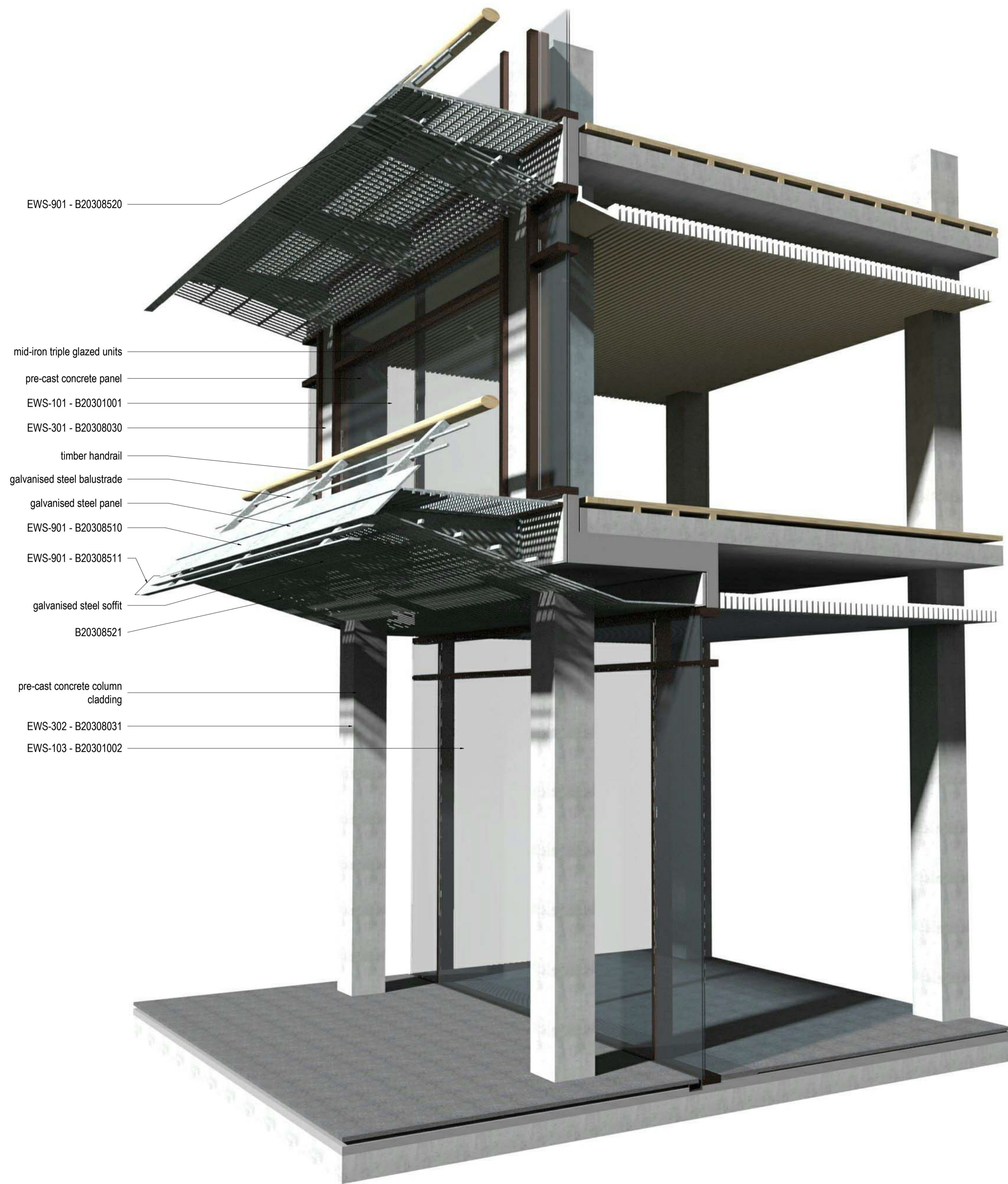
01 Sectional Perspective - Ground Floor NTS @ A1
