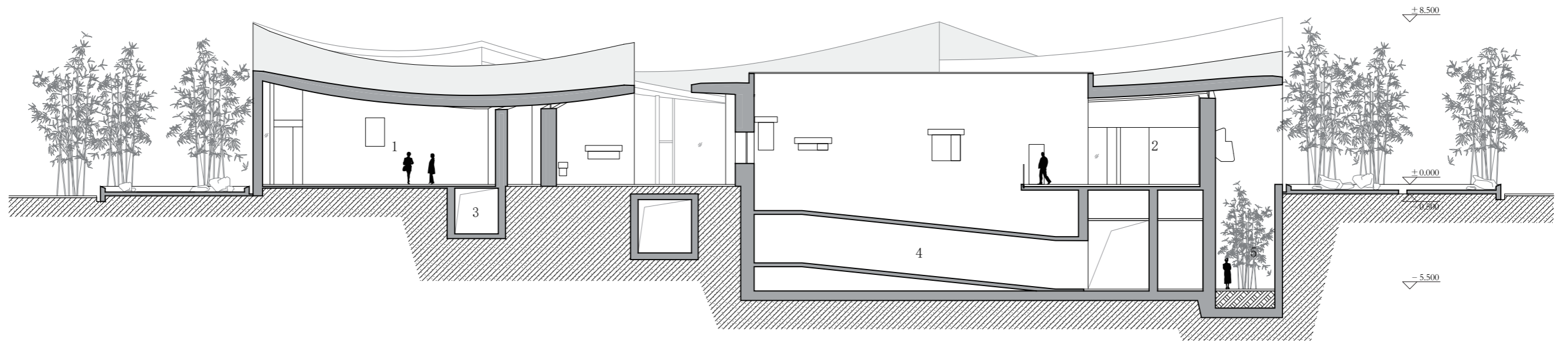
Section 2-2
