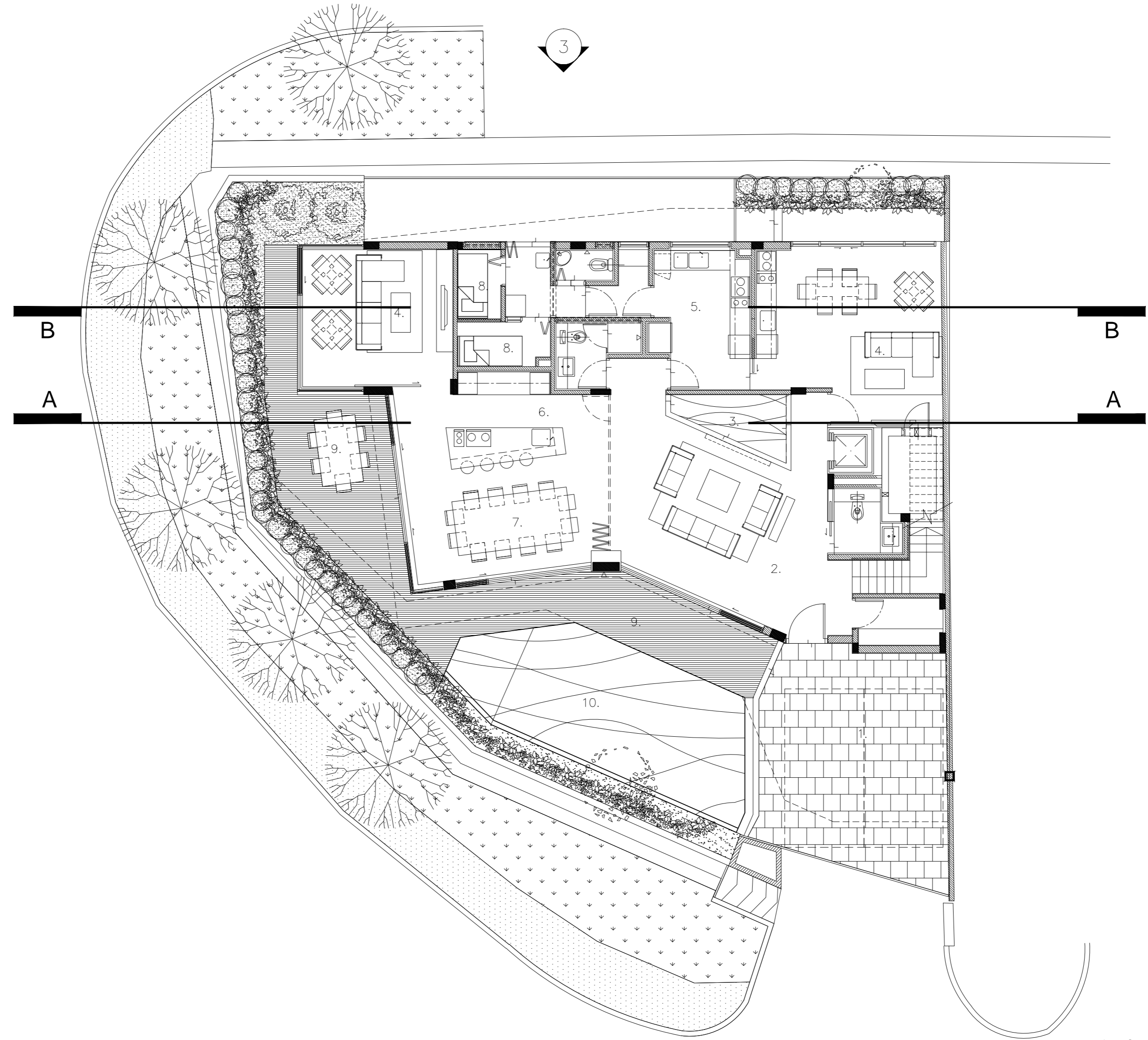
1st STOREY PLAN 0 2 4 6 8 10 METRES
