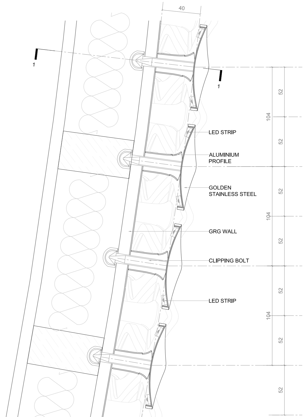
LEAF COMPONENT SECTION
