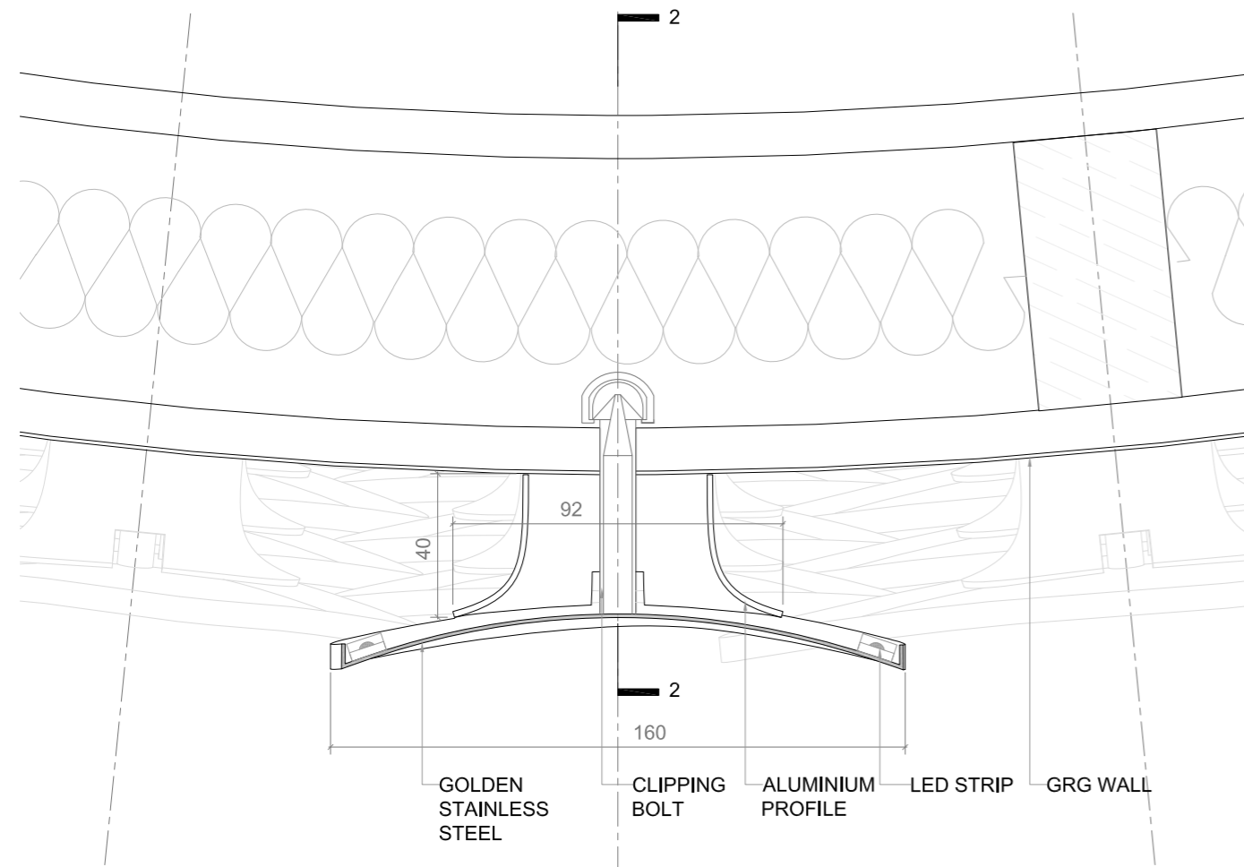
LEAF COMPONENT PLAN
