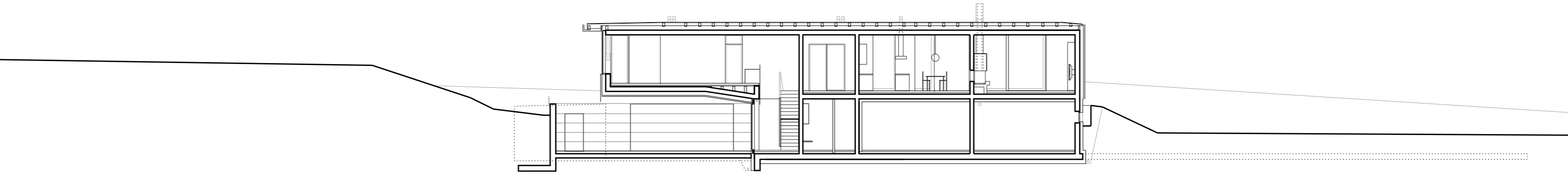
1-1 1:200
