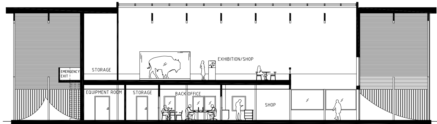
LONGITUDINAL SECTION PRINCIPLE Scale 1:100 (A1)
