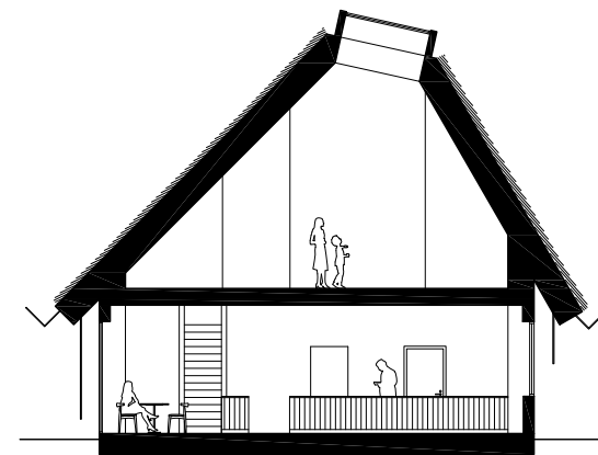
CROSS-SECTION PRINCIPLE Scale 1:100 (A1)
