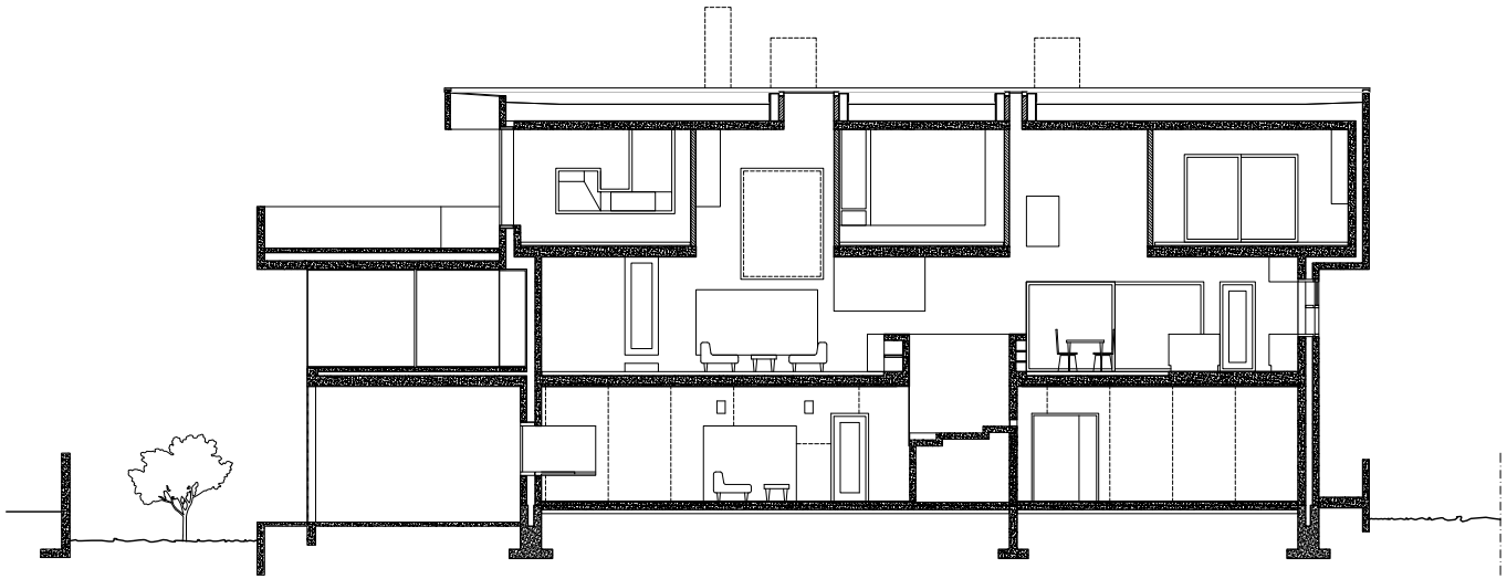
LONG SECTION 1:200/A4
