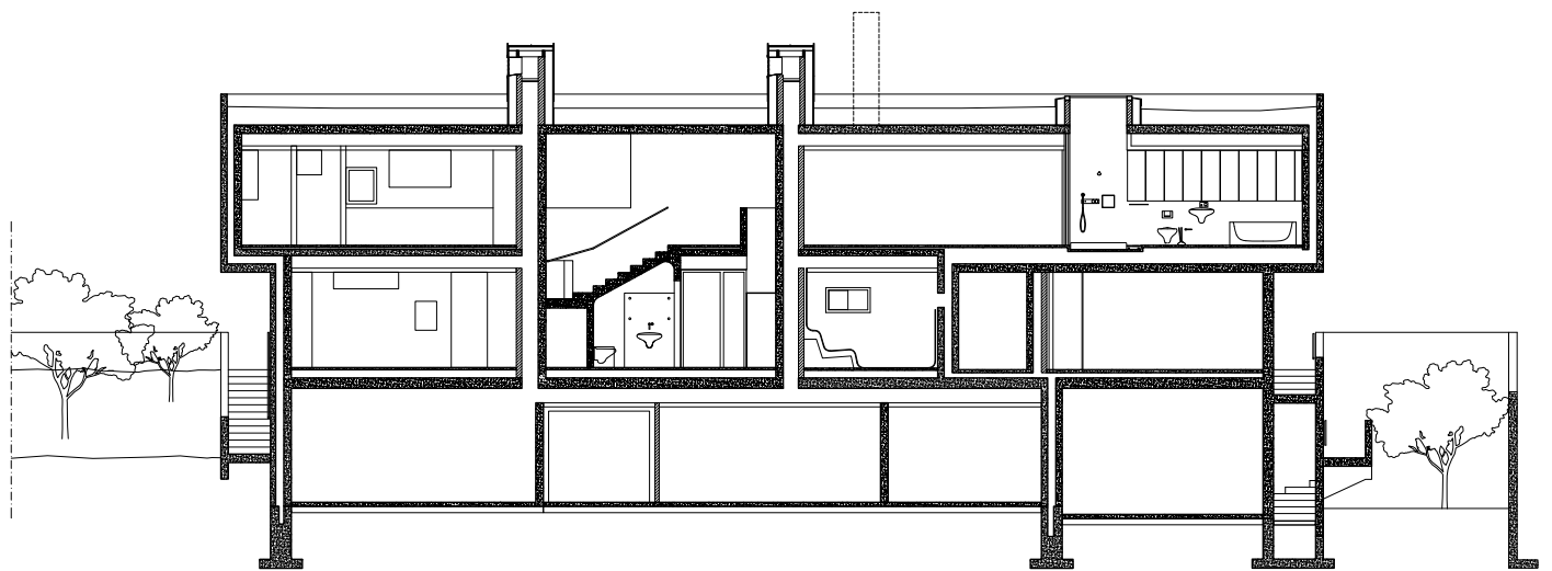
LONG SECTION 1:200/A4
