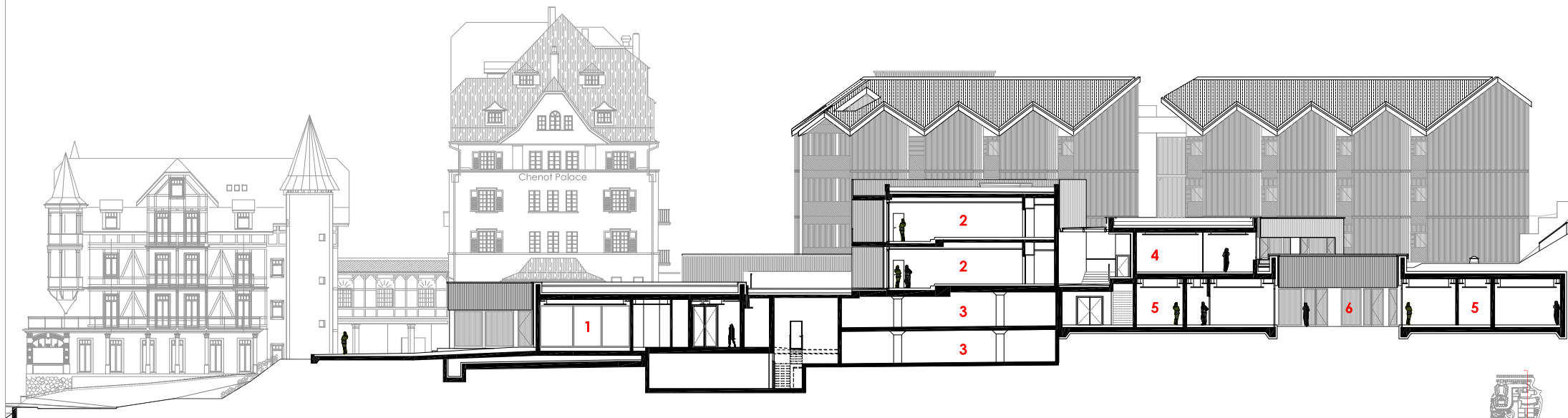
LONG SECTION
