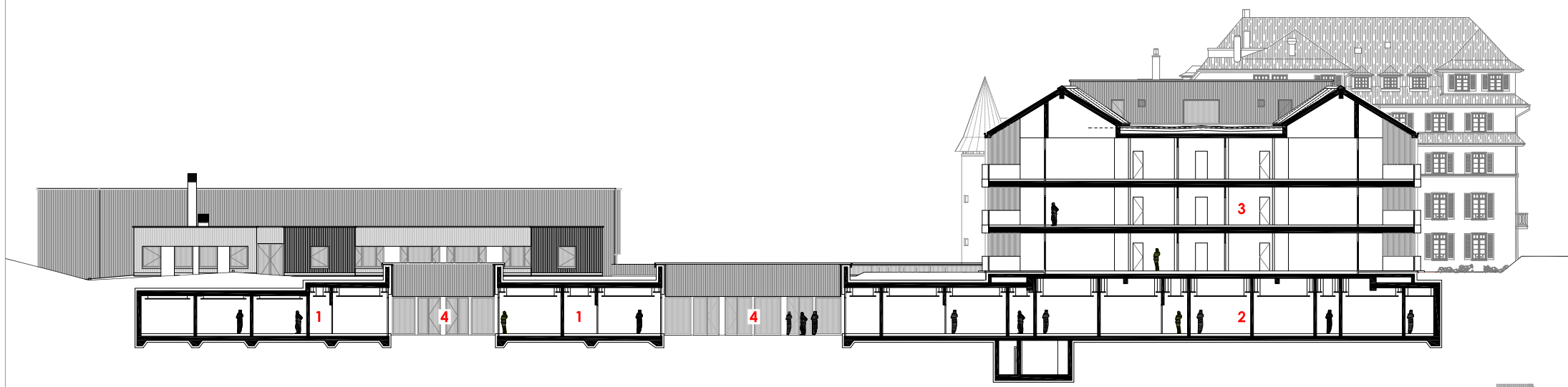
CROSS SECTION
