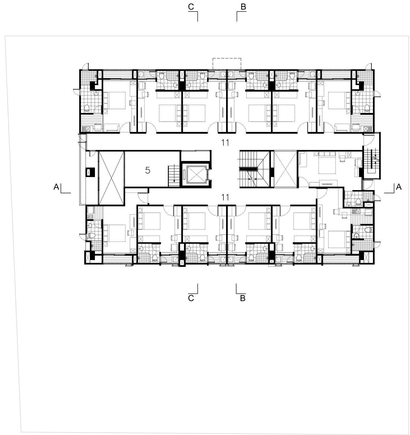
N THIRD FLOOR PLAN
