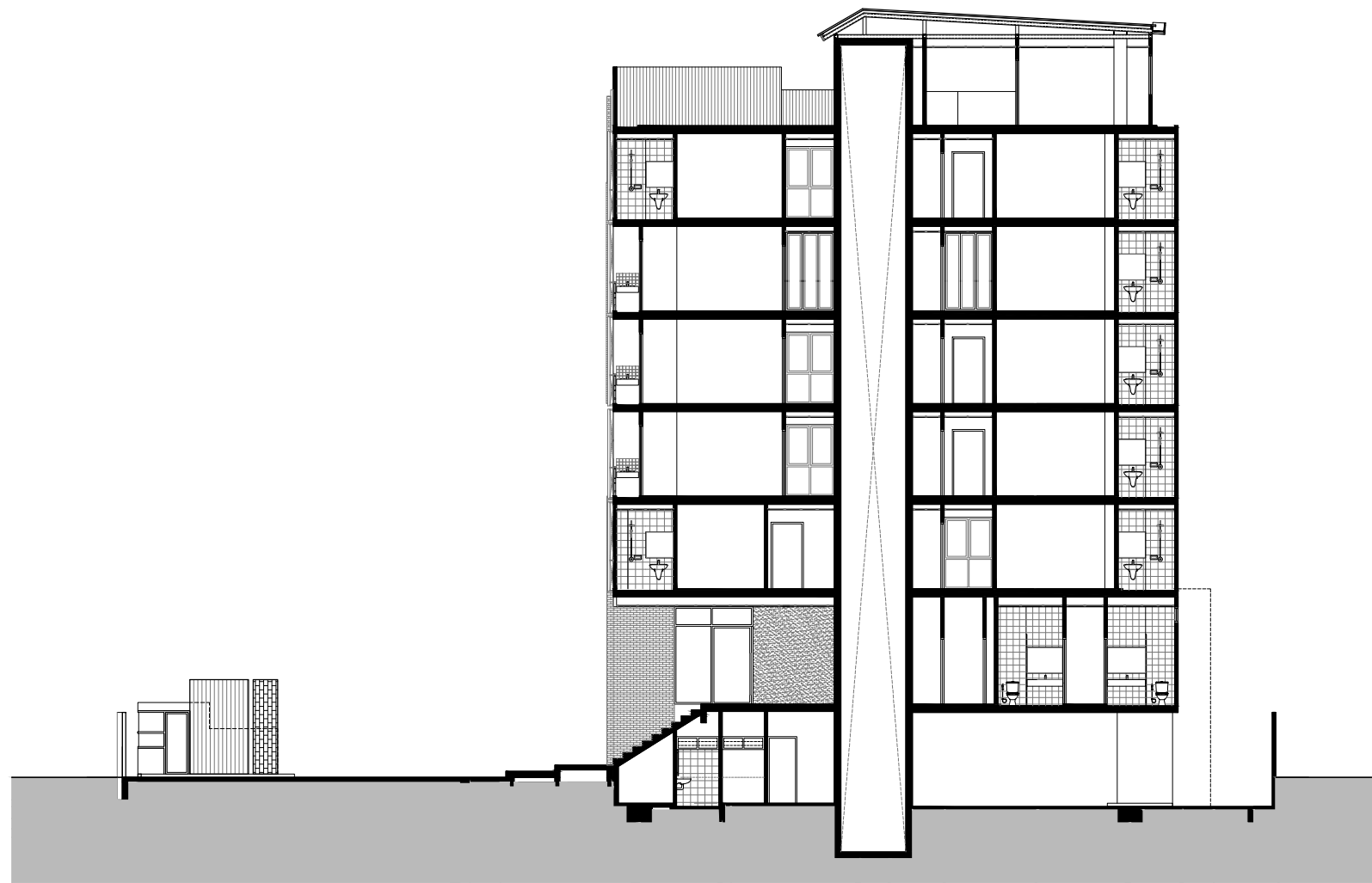
C-C SECTION
