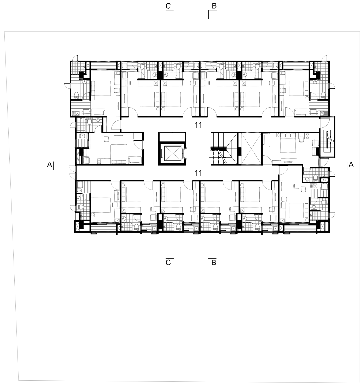
N SEVENTH FLOOR PLAN
