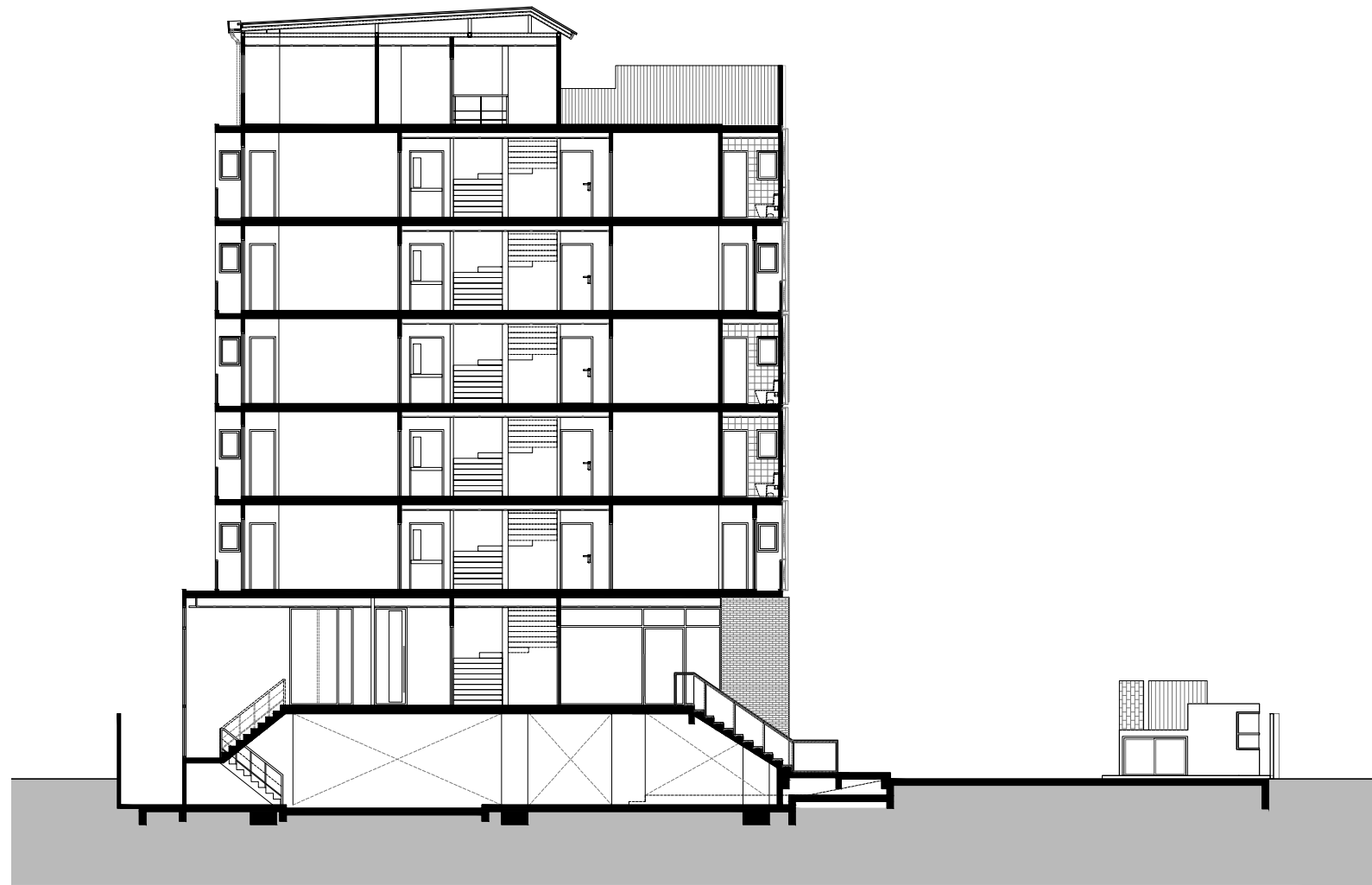
B-B SECTION
