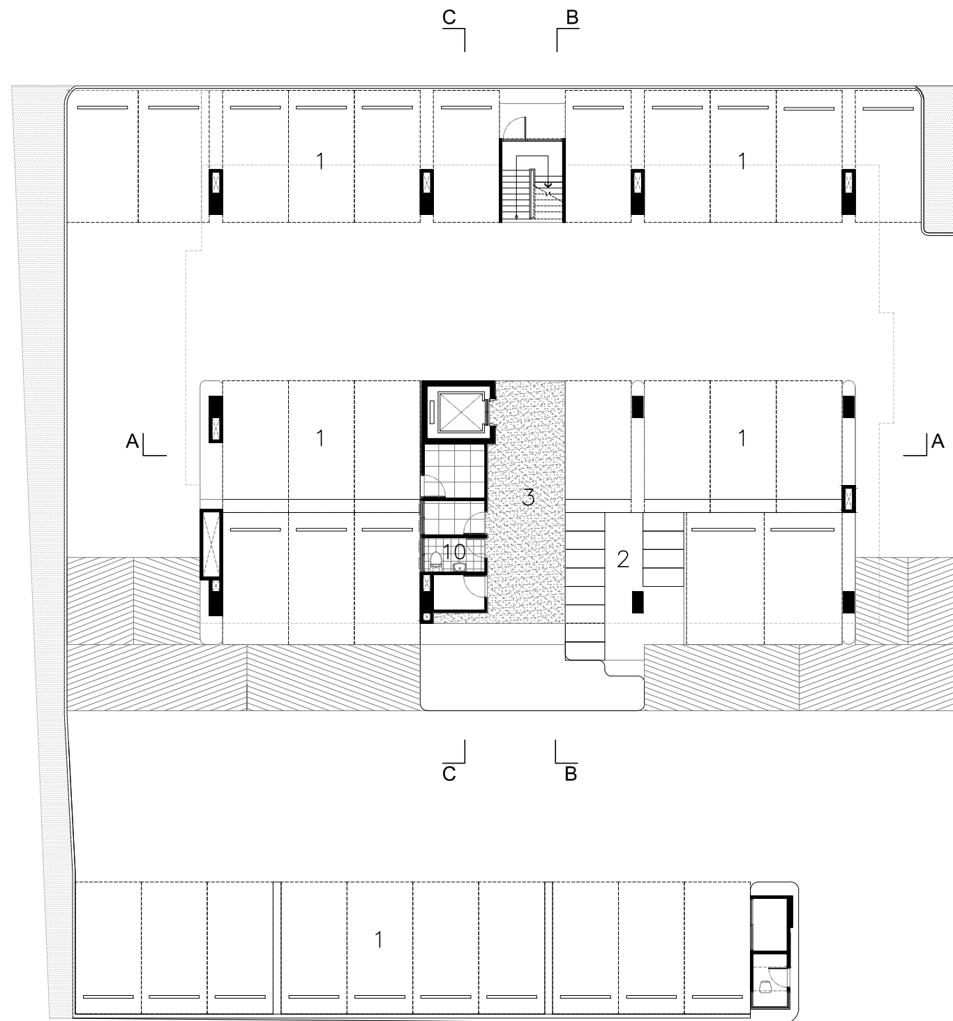
N BASEMENT - FIRST FLOOR PLAN
