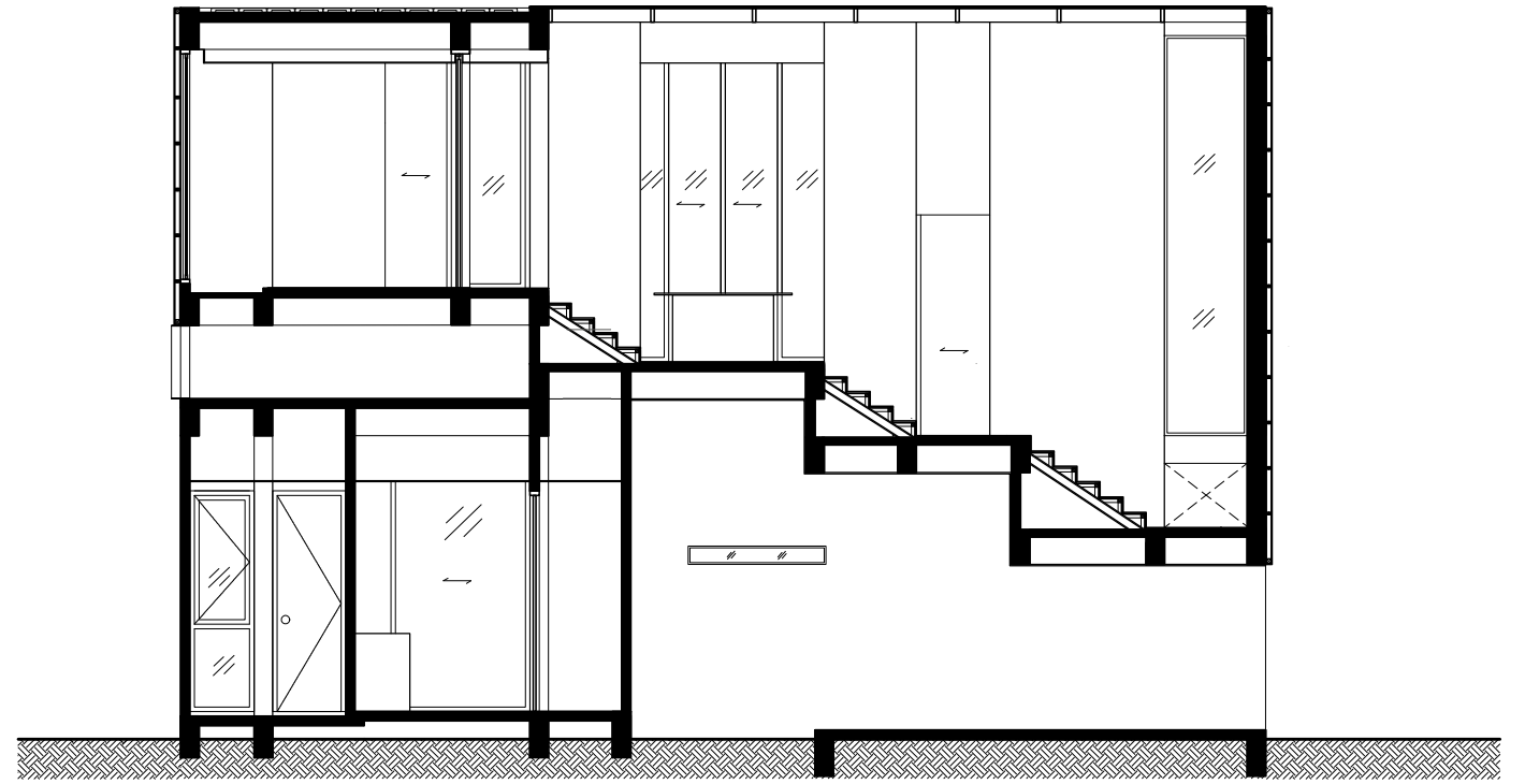
SECTION 2
