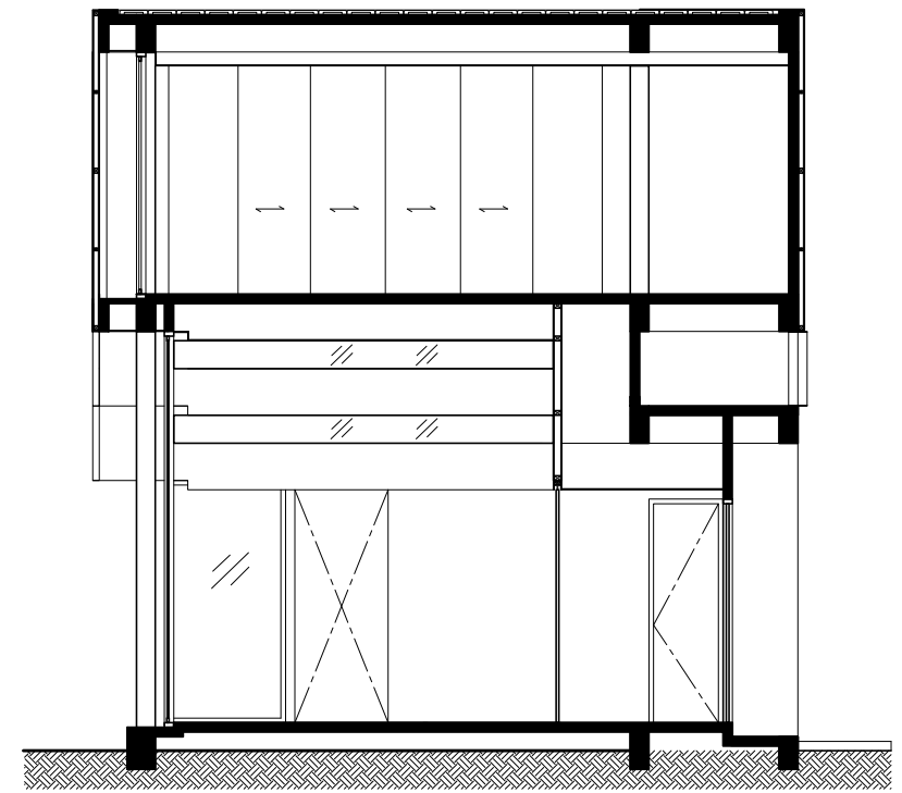
SECTION 4
