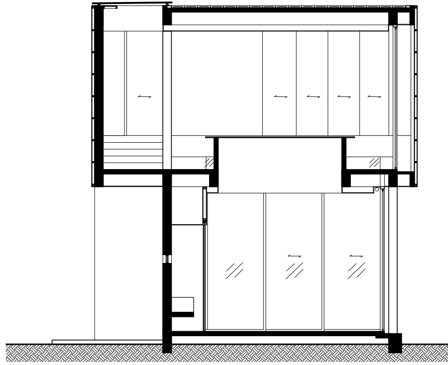
SECTION 1
