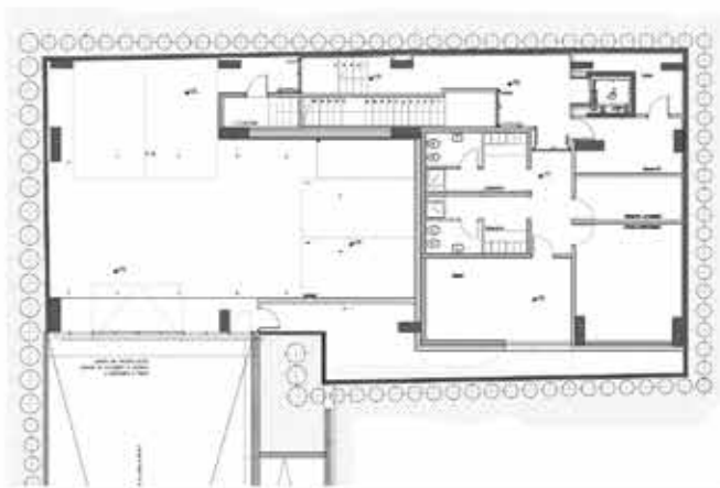
Piano interrato
