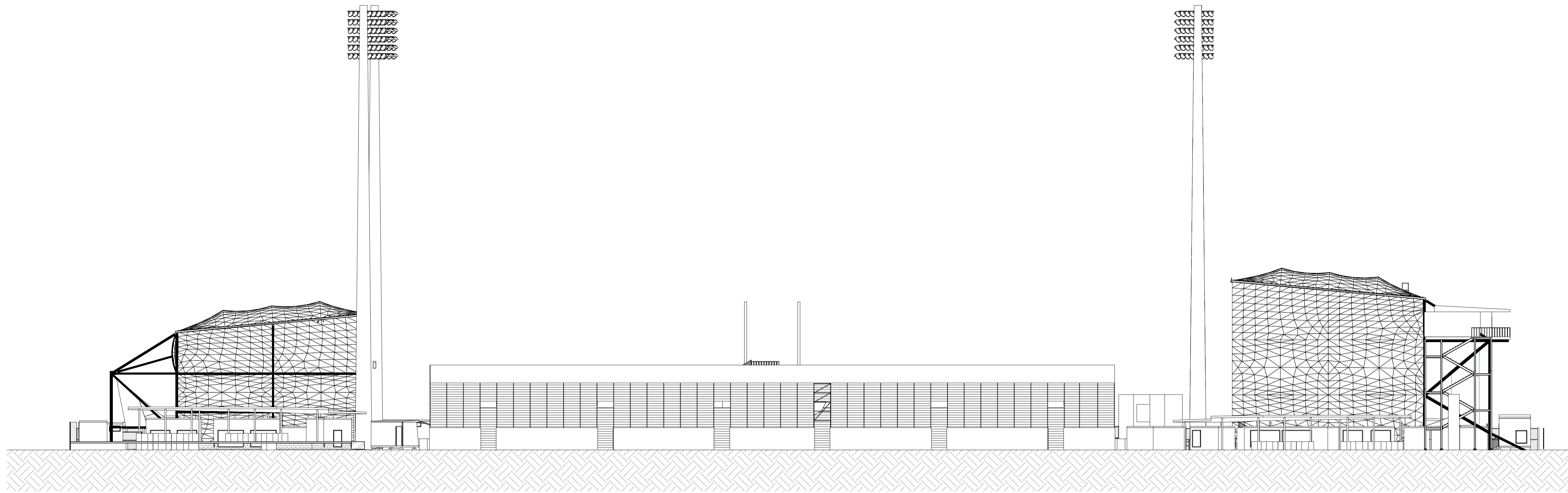
1 EAST ELEVATION 1 : 250
