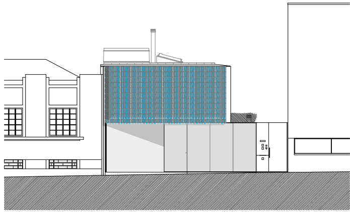
STREET ELEVATION
